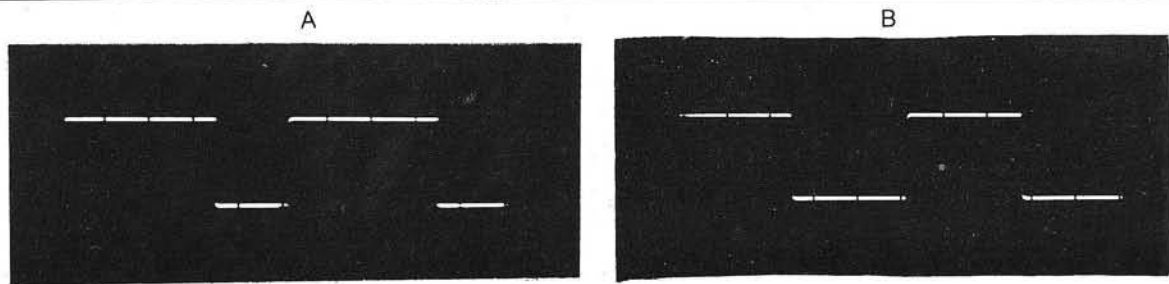
Figure 5: Oscilloscope traces showing relationship of R_a , R_b and the output waveform. At A, R_a = R_b and the output is high twice as long as it is low. At B, R_a = 0 and the high pulse is the same length as the low pulse.
