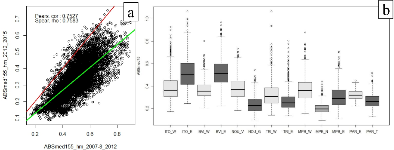
Fig. S4. a) Annualized canopy dynamics during two successive periods (here 2007-8_2012 and 2012_2015 - NOU) show strong spatial correlation (green); lower values at the second period are attributed to instrumental differences; b) Distribution per site of ABSmed75 indicator of canopy dynamics (one ha cells)
