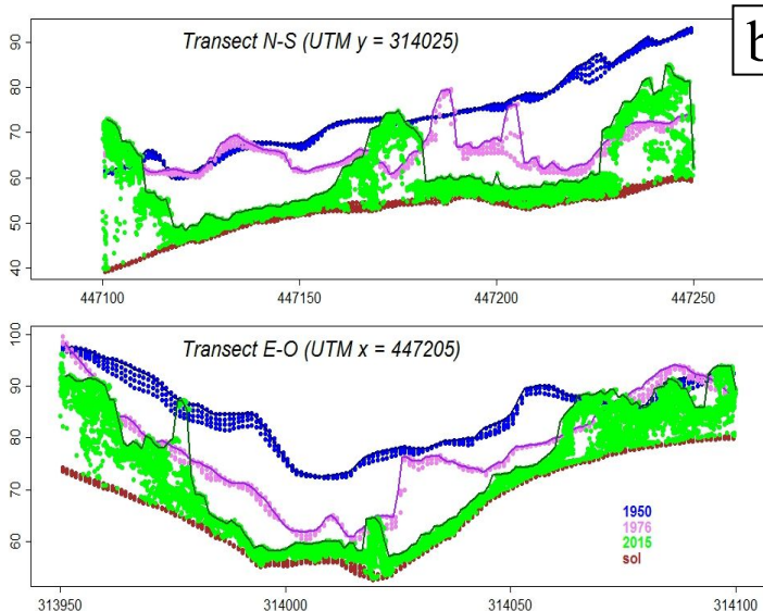
Fig. S10. a) A comparison of canopy height models (CHM) derived from LiDAR (2015) and photogrammetry (1950, 1976) showing the appearance of a bamboo patch ; above : CHM 1950 / 1976 / 2015 ; below : ortho-photos 1950 / 1976 et Pléiades image 2014 ; b) North-South and East-West Transects of 1950, 1976 et 2015 CHMs ; low vegetation are bamboos.
