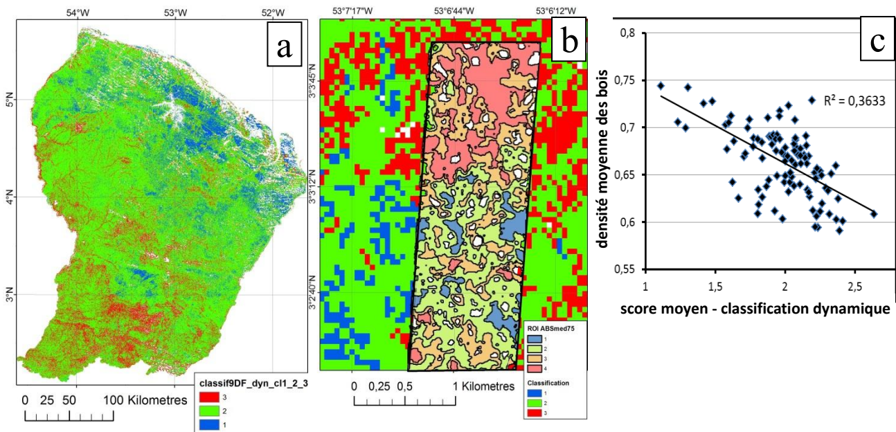
Fig. 58. a) Supervised classification of Landsat mosaic in three classes of dynamics; b) Training areas (“ROI-dynamics”) in 4 classes of the indicator ABSmed75 (see Fig. 3b) overlaid over classification following fusion of classes 3 and 4; ITO-north-west; c) Relation between wood density (WSG) and dynamics scoring (Habitats data and Landsat derived forest dynamics map).
