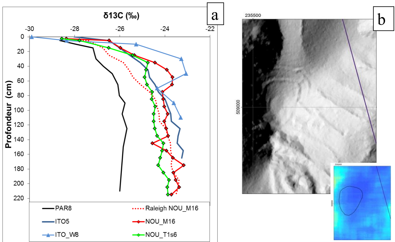
Fig. S11. a) Sample \delta^{13}\text{C} profiles of soil organic matter; PAR8 and ITO5 show extreme variations covering the range of variation attributable to soil characteristics alone; ITO_W8, NOU_M16 and _T1s6 conversely show a more or less pronounced deviation from the theoretical model (Raleigh), represented by NOU_M16; b) Geoglyphe with double ditch and flat top in Mt de la Trinité, TRI_W, dynamics 2014-16.
