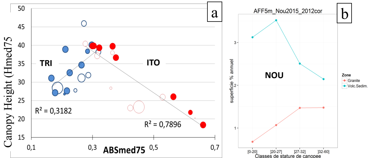
Fig. S9. a) Examples of contrasting canopy height- canopy dynamics relation (Hmed75 ~ ABSmed75) in TRI and ITO ; solid bubbles : deep soils ; empty bubbles : thinned soils ; bubble size proportional to deviation to the site mean soil depth; b) Contrasting dynamics associated to different geological substrates in NOU (annual percentage of canopy affected by a subsidence event greater than 5 m plotted per forest height class).
