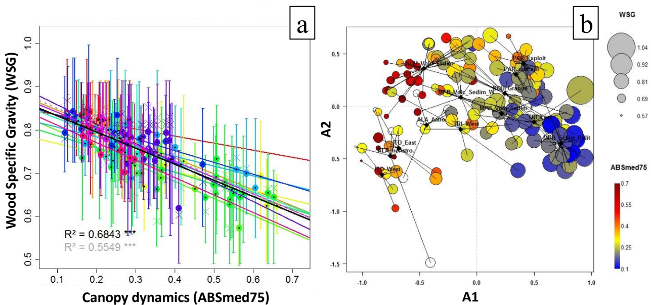
Fig. S5. a) Linear correlation between WSG and canopy dynamics (colour : site ; dot : mean value per sample; cross : median value per sample; whiskers: interquartile ; r^2 of global linear regression (black : mean values, grey : median values); b) Bray-Curtis floristic similarities projected using Non Metric Multidimensional Scaling (NMDS) additionally showing Wood Specific Gravity (WSG) and local dynamics (ABSmed75).
