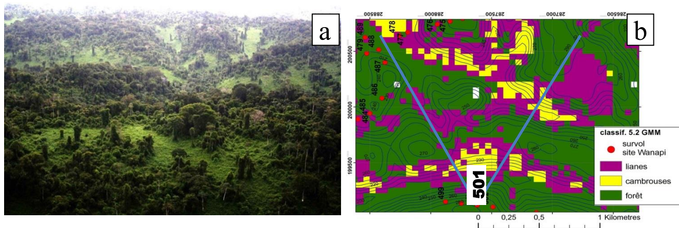
Fig. S7. a) Open canopy landscape in Wanapi showing cambrous and lianas (photo n° 501 D. Sabatier); b) Corresponding extract of the vegetation map derived from landsat mosaic. Lines show the approximate field of view of photo 501.
