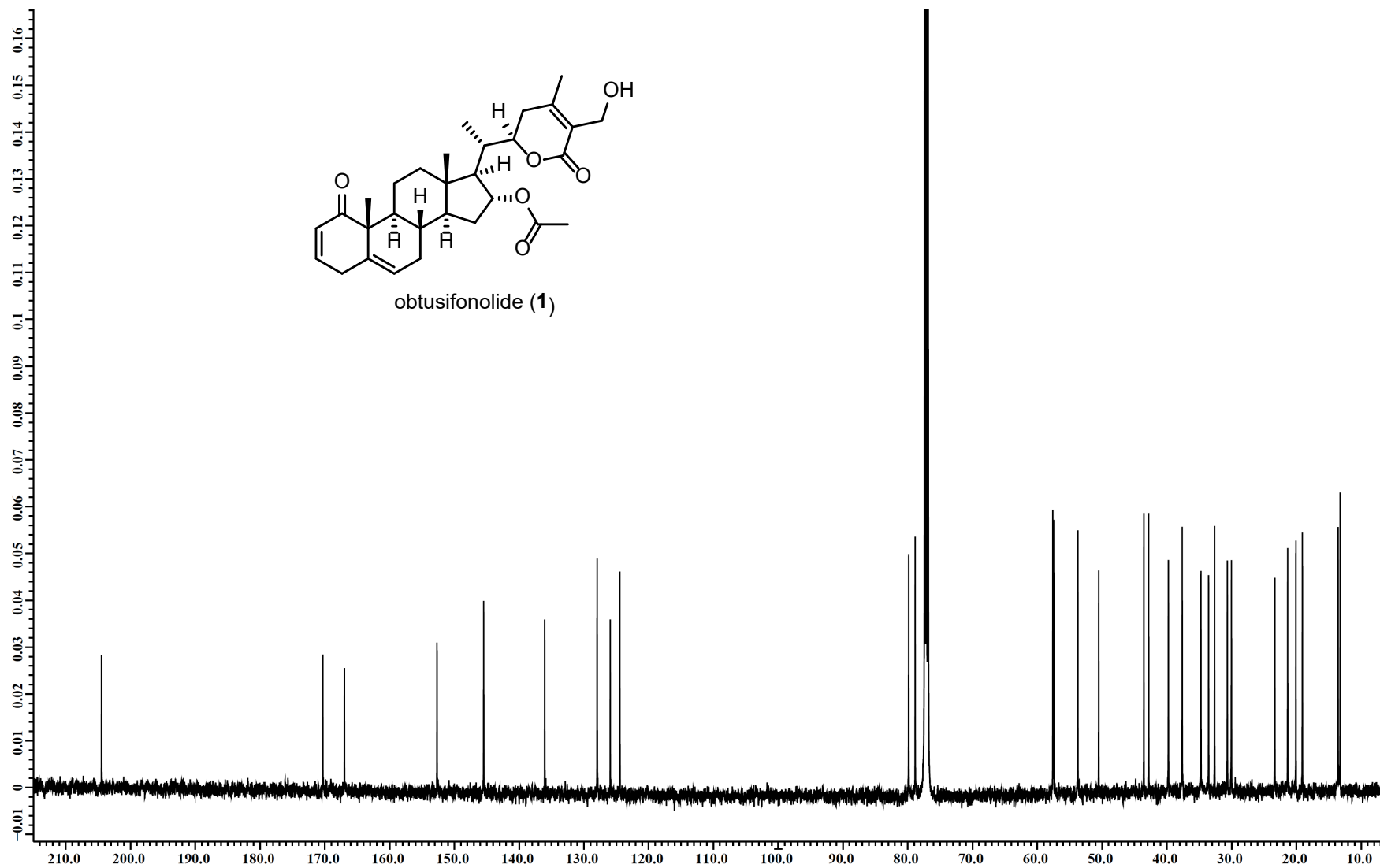
Fig. S3. 13 C NMR spectrum of obtusifonolide (1) [125 MHz, CDCl 3 ].
