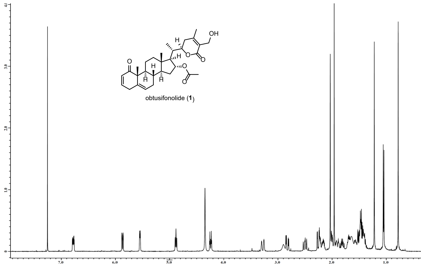
Fig. S2. 1 H NMR spectrum of obtusifonolide (1) [500 MHz, CDCl 3 ].
