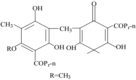
Filicic acid
