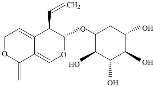
Gentiopicrosin
