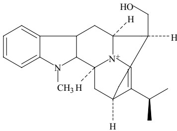
Fig. 17.19 Structure of Alstoumerine.
