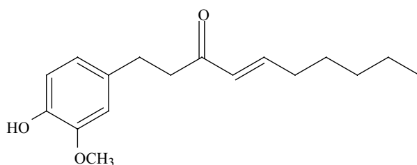
[6]-shogaol
