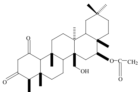
Fig. 14.10 Structure of kotalagenin 16-acetate.
