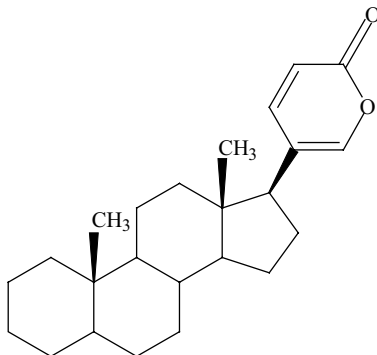
Fig. 5.143 Structure of bufadienolide.
