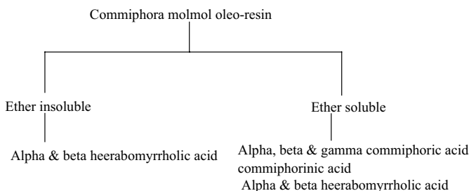
Fig. 5.203 Oleoresin of Commiphora molmol .
