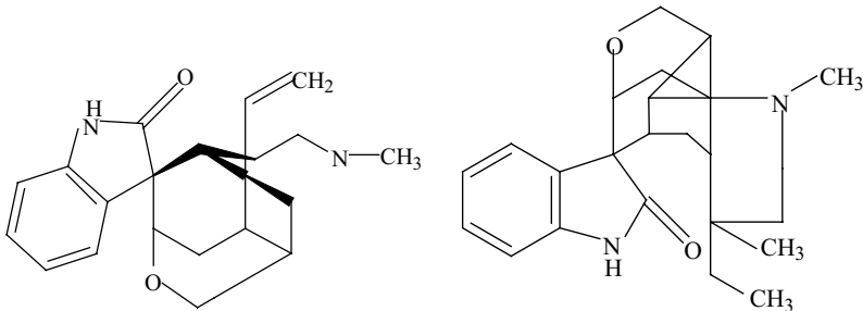
Fig. 5.75 Structure of Gelsemine and Gelseminine.
