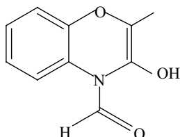
Fig. 5.56 Structure of Cappamansin A.
