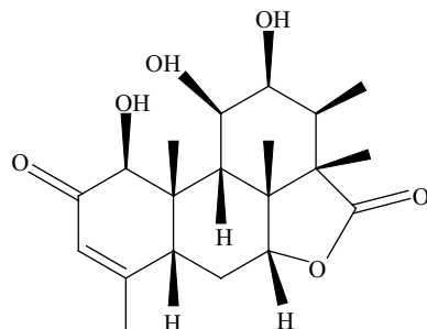
Fig. 5.109 Structure of 11-Dehydroklaineaneone.
