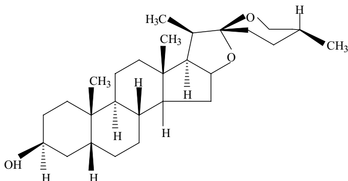
Fig. 5.172 Structure of Sarsasapogenin.
