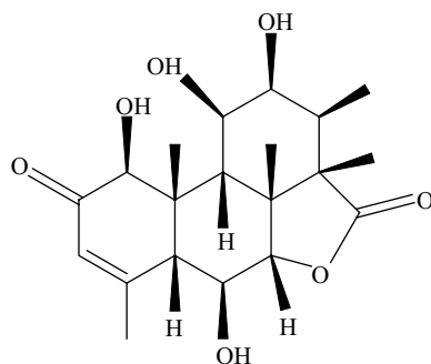
Fig. 5.108 Structure of Longilactone.
