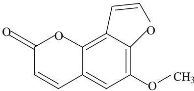
Sphondin
