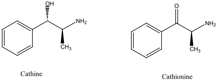
Fig. 5.74 Structure of Cathine and Cathionine.
