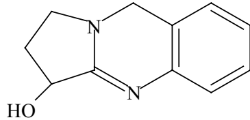
Vasicine
