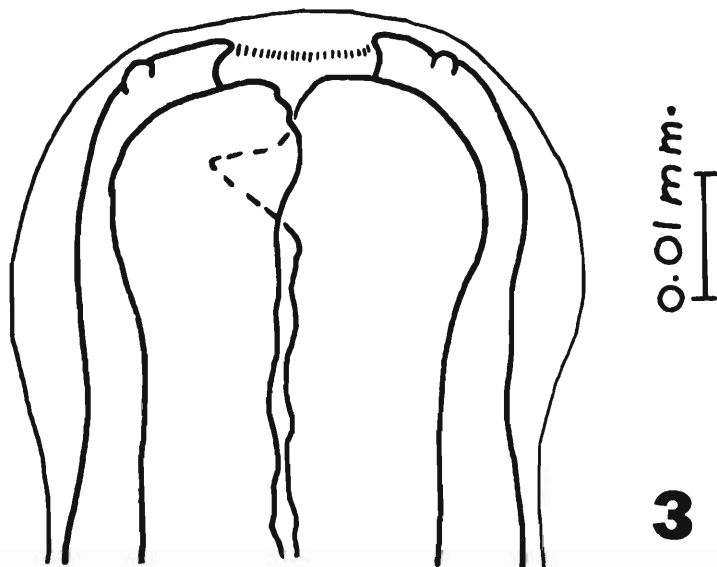
Fig. 3. Nematodirus helveticus (male): Cephalic and stomatal regions in lateral view, showing large dorsal esophageal tooth.
