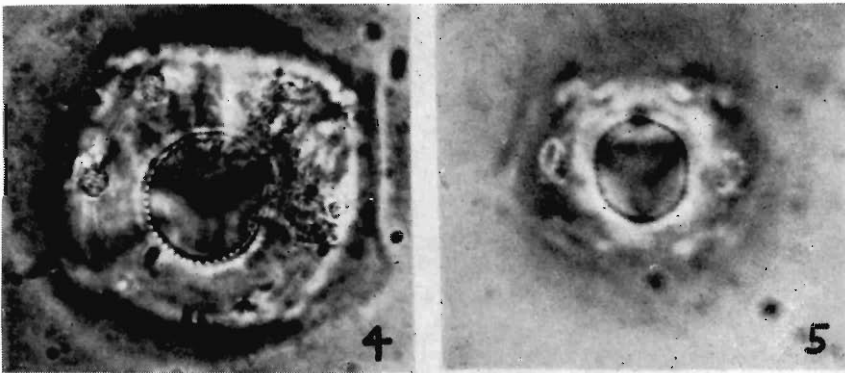
Fig. 4. Nematodirella longispiculata (male): Photomicrograph of head, en face . (147X).
