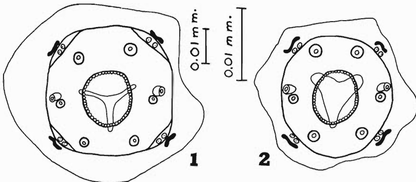
Fig. 1. Nematodirella longispiculata (male): Head, en face .
