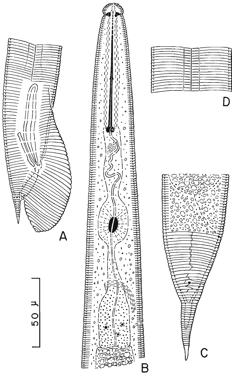
Figure 1. Dolichodorus similis , n. sp. A. Posterior portion of male in lateral view. B. Anterior portion of female. C. Posterior portion of female. D. Lateral field as usually found on female slightly anterior to vulva.
