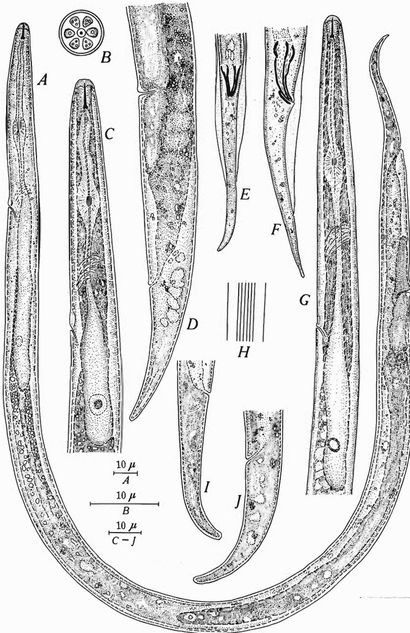
Fig. 2. Pseudhalenchus anchilispomus . A, B, F, and G. Specimens from Berkeley, California. A. Adult female. B. Female face view. F. Lateral view of male tail. G. Esophageal region of female. C-D. Female specimens from Deland, Florida. C. Esophageal region. D. Posterior portion of body. E. Ventral view of tail, male from Ocala, Florida. H. Lateral field at middle of body, female from West Jordan, Utah. I, J. Tails of females from Lodi, California.
