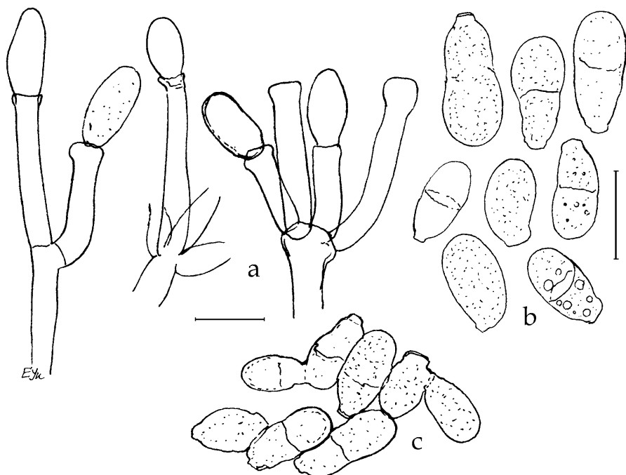
Fig. 1. The anamorph of Hypomyces aurantius ( Cladobotryum varium ) from culture: a – conidiophores with conidia (MSK 8486), b – conidia (MSK 8518), c – agglutinated and anastomosed conidia (MSK 8518). Scales = 10 \mu\text{m} .
