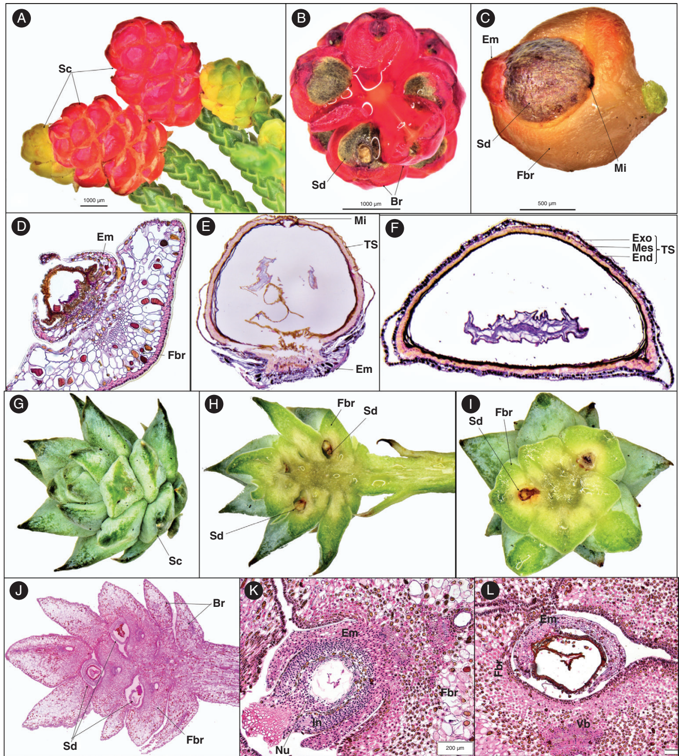
FIG. 3. Seed cone morpho-anatomical features of Microcachrys (A–F) and Saxeogethaea (G–L) showing: (A) fleshy red and young yellowish seed cones; (B) seed cone cross-section view showing seed (Sd) and bract (Br); (C) seed cone with epimatium (Em), seed (Sd), fertile bract (Fbr) and micropyle (Mi); (D) young ovule development (post-pollination) shows fertile bract, epimatium and ovule (Ov); (E) longitudinal section of single seed cone showing testa (TS), micropyle (Mi) and epimatium; (F) seed cone cross-section showing the different layer of testa, i.e. exotesta (Exo), mesotesta (Mes) and endotesta (End); (G) seed cone (Sc); (H) seed cone longitudinal section showing fertile bract (Fbr) and seed (Sd); (I) cross-sections showing the seed cone with the fertile bract and seed; (J) longitudinal section of seed cone showing fertile bract, seed and bract; (K) longitudinal section of developing ovule (post-pollination) showing epimatium, nucellus (Nu), fertile bract and integument (In); and (L) cross-section of developing ovule (post-pollination) showing epimatium, fertile bract and vascular bundle.
