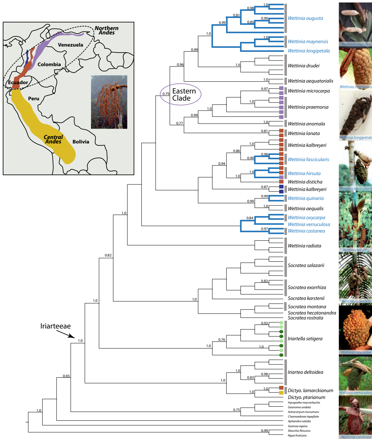
Figure 1. Phylogenetics of the palm tribe Iriarteeae estimated using Bayesian inference implemented in BEAST. Clade support > 0.75 (Bayesian posterior probability) is displayed to the upper left of each node. Species are indicated with a grey bar when multiple individuals were sampled and those with a tightly packed infructescence are shown in blue font and branches. The insert map shows the location of the central and northern Andes and the three cordilleras of the northern Andes, in which dark blue is the western, orange is the central and purple is the eastern Cordillera. Andean taxa are indicated with squares at tips with colours reflecting in which Cordillera they occur. A loosely arranged infructescence of Wettinia disticha is shown to contrast with the tightly packed morphology, which is shown to the right of the tree. Dictyocaryum is abbreviated Dictyo. and light and dark green circles represent individuals of Iriartella setigera and I. stenocarpa , respectively.
