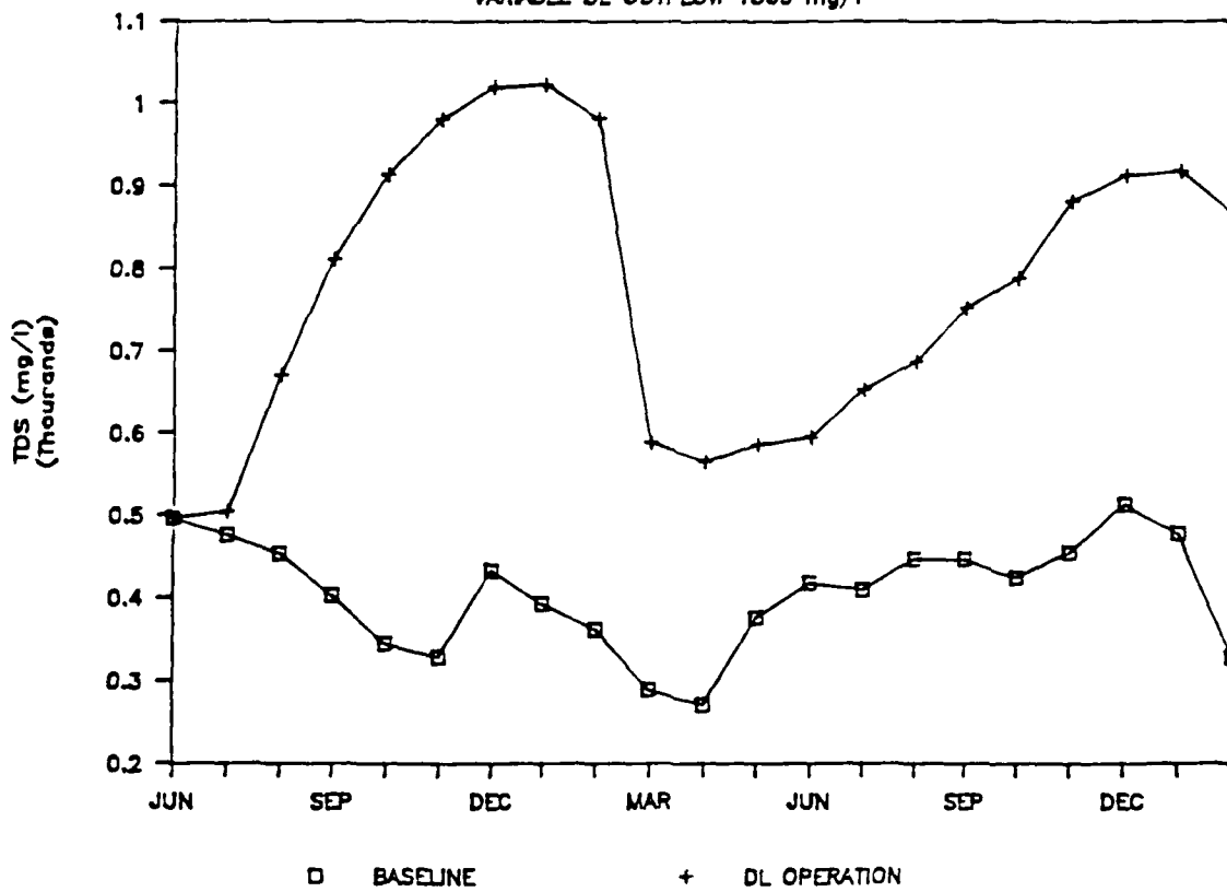
FIGURE 11 SHEYENNE R. AT KINDRED, ND VARIABLE DL OUTFLOW 1500 mg/l
