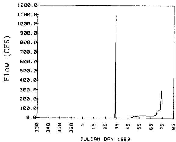
Figure 19, Discharge from Connecting Channel in 1982-83 Winter
