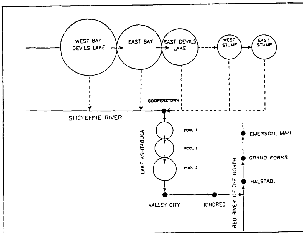
FIGURE 2 - DEVILS LAKE - SHEYENNE RIVER - RED RIVER OF THE NORTH MODEL CONFIGURATION
