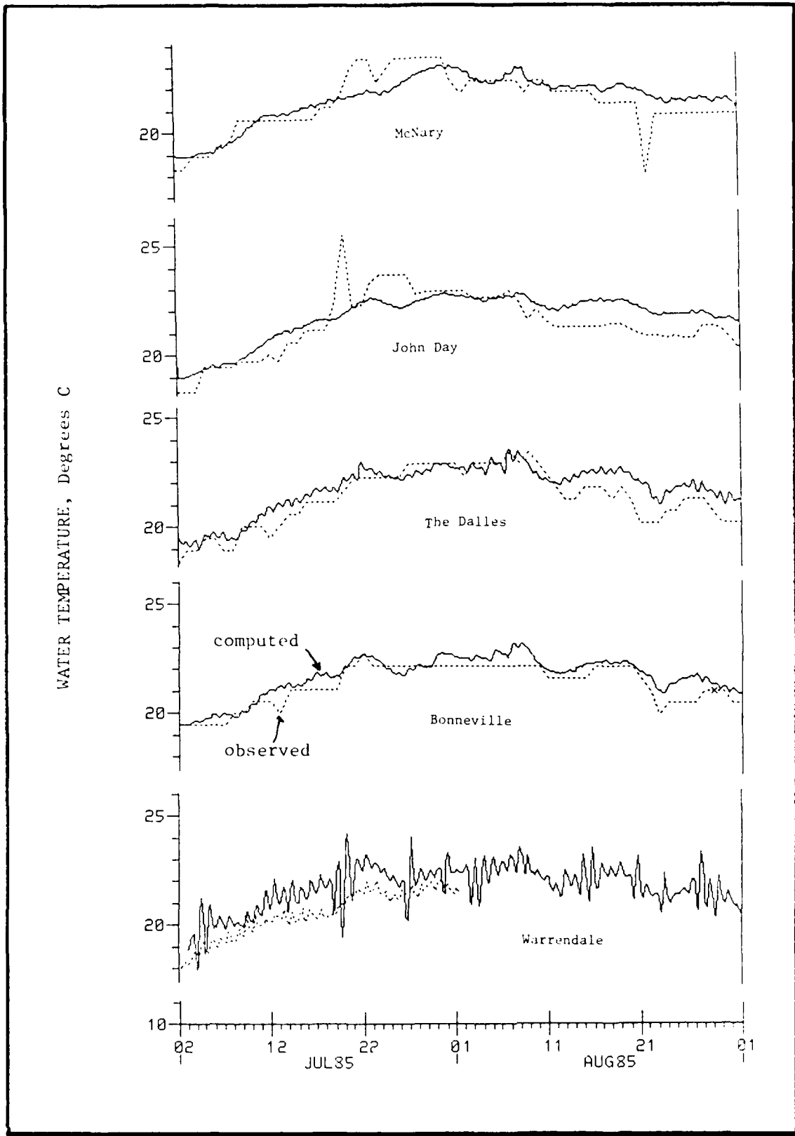
Figure 8. Model Calibration for 1985 : Lower Columbia
