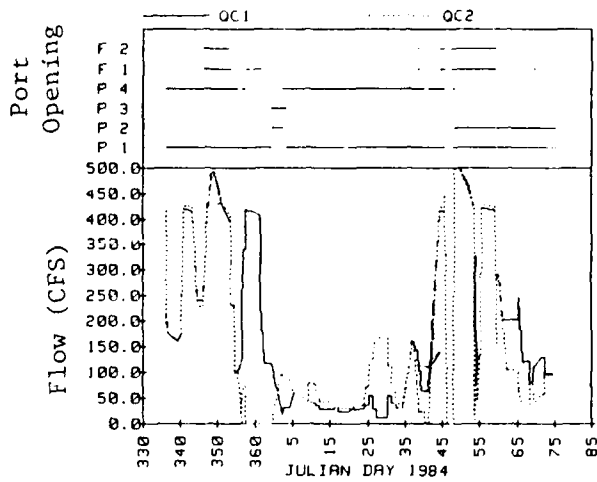
Figure 25, Discharge from Tioga QC Gates and Portal Opening
