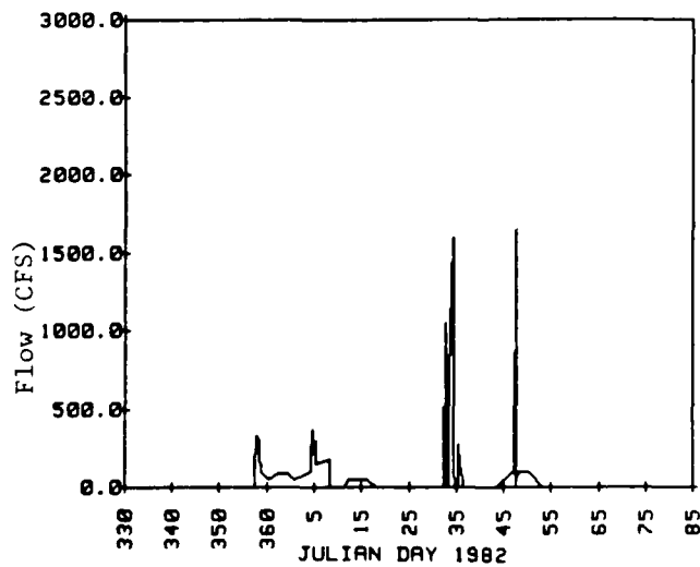
Figure 15, Discharge from Connecting Channel Gates in 1981-82 Winter
