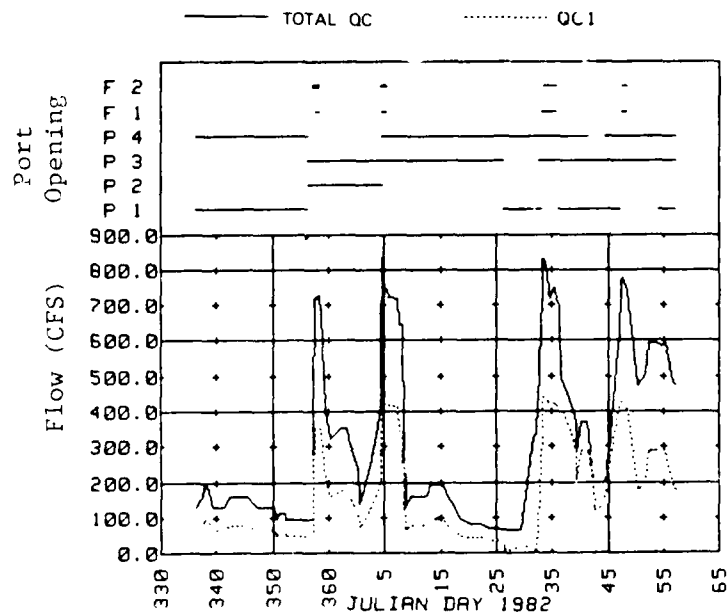
Figure 12, Discharge from Tioga QC and Portal Opening in 1981-82 Winter
