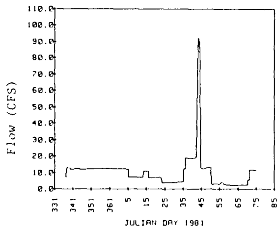
Figure 11, Discharge from Crooked Creek Outlet Works 1980-81 Winter
