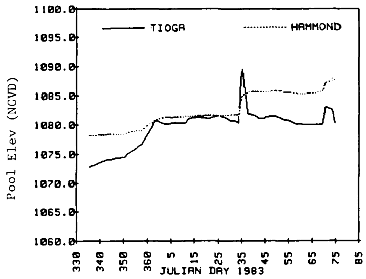
Figure 17, Pool Elevations in 1982-83 Winter
