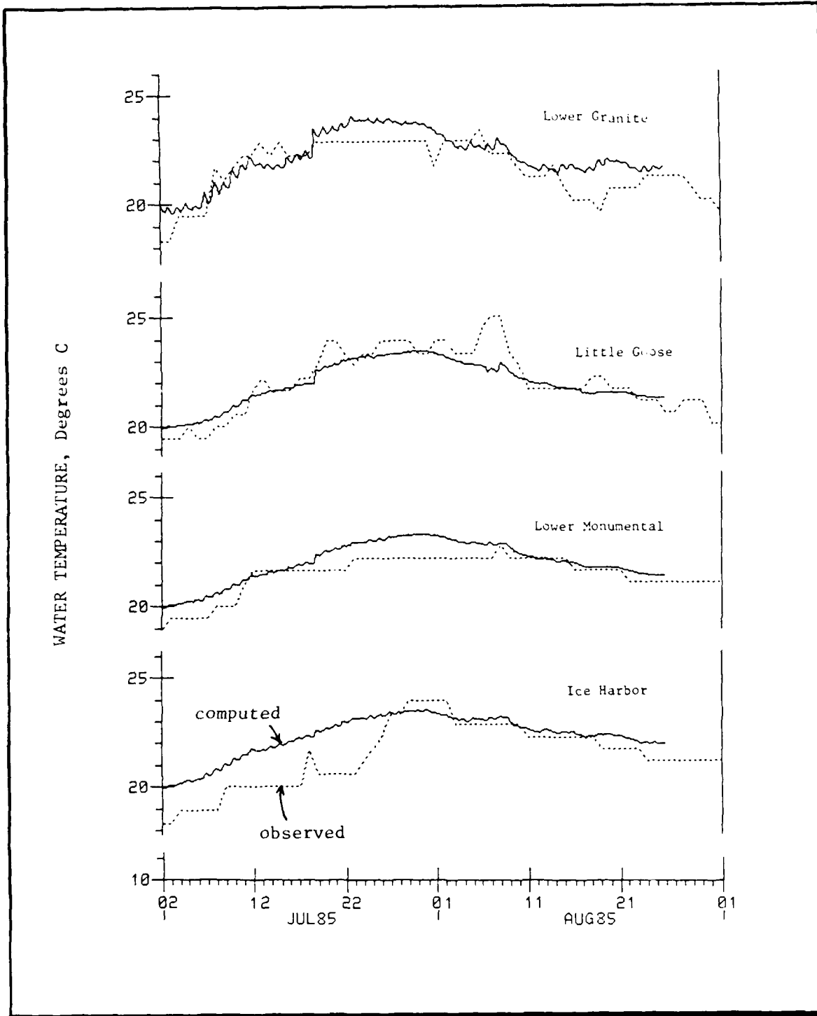
Figure 7. Model Calibration for 1985 : Snake
