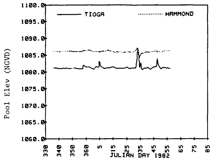
Figure 16, Pool Elevations in 1981-82 Winter
