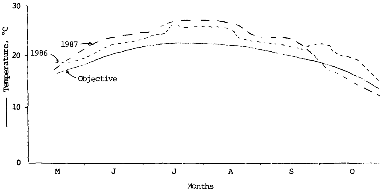
Beech Fork Lake Outflow Temperatures
