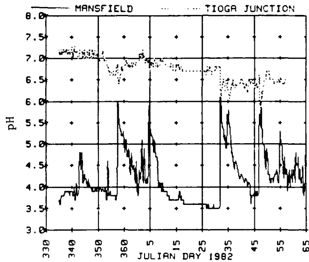
Figure 14, Inflow and Outflow pH in 1981-82 Winter
