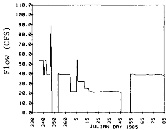
Figure 32, Discharge from Crooked Creek Outlet Works 1984-85 Winter
