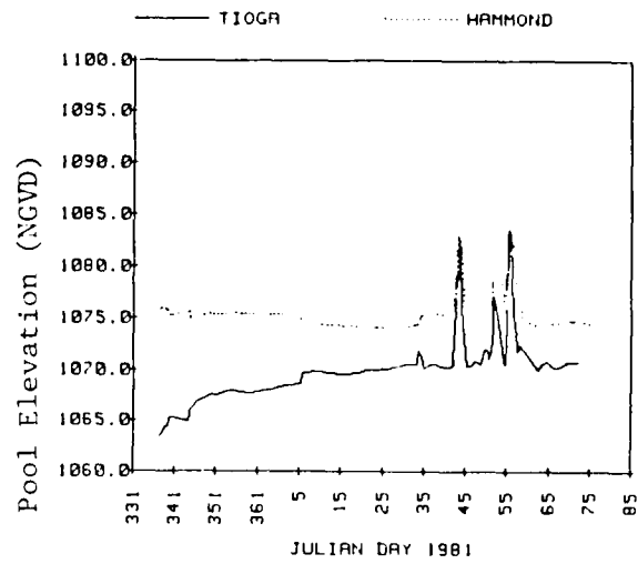
Figure 10, Pool Elevations in 1980-82 Winter
