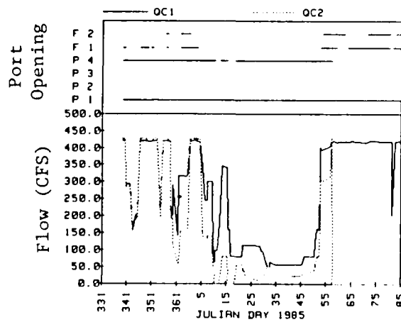
Figure 33, Discharge from Tioga QC Gates and Portal Opening in 1984-85 Winter
