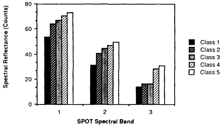
Figure 5. Mean values of the five multispectral signatures.
