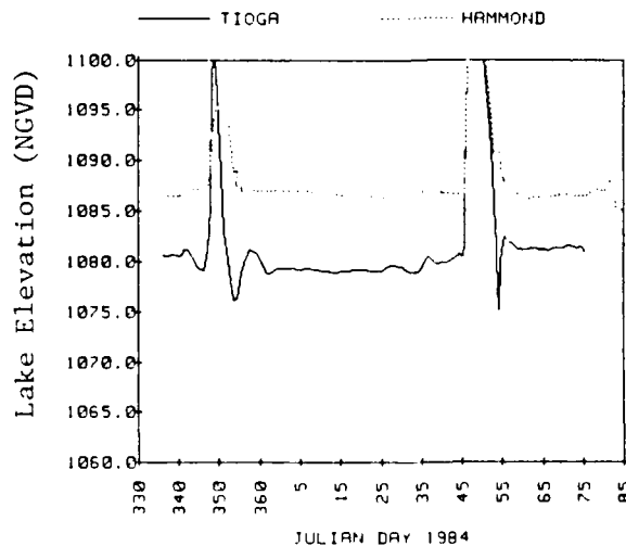
Figure 23, Lake Elevations in 1983-84 Winter
