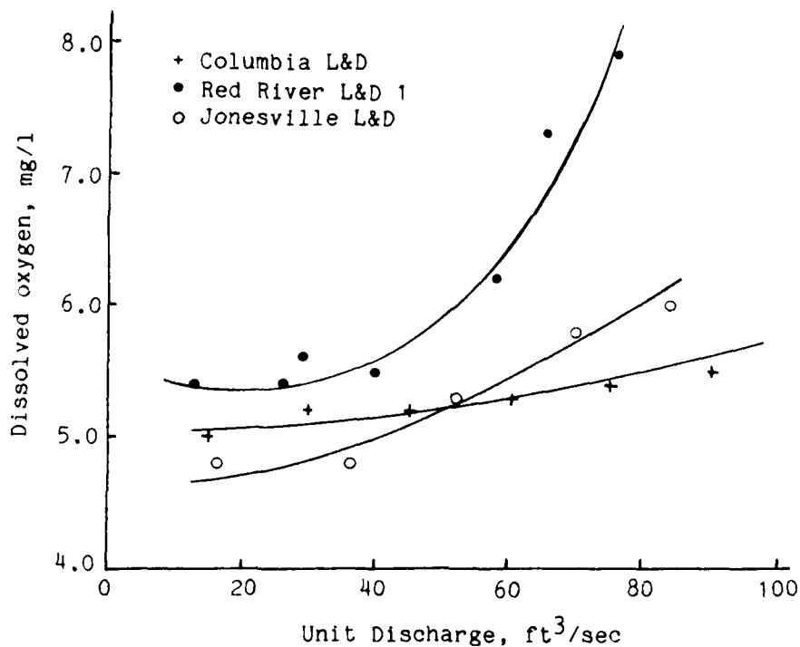
Figure 2. Release dissolved oxygen versus release flow rate.
