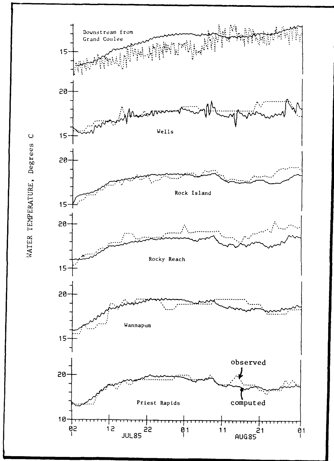
Figure 6. Model Calibration for 1985: Upper Columbia
