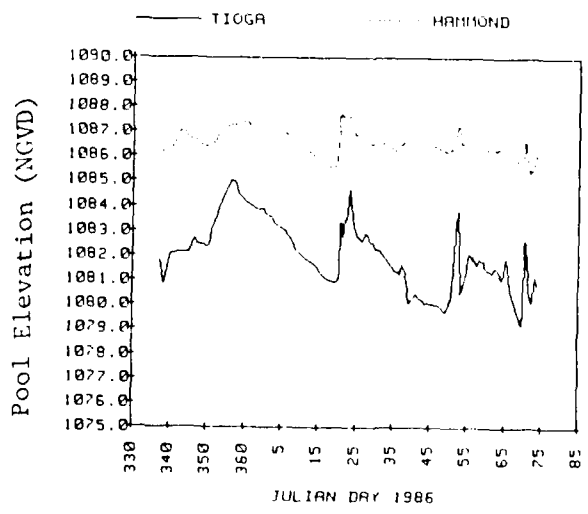
Figure 45, Pool Elevations in 1985-86 Winter
