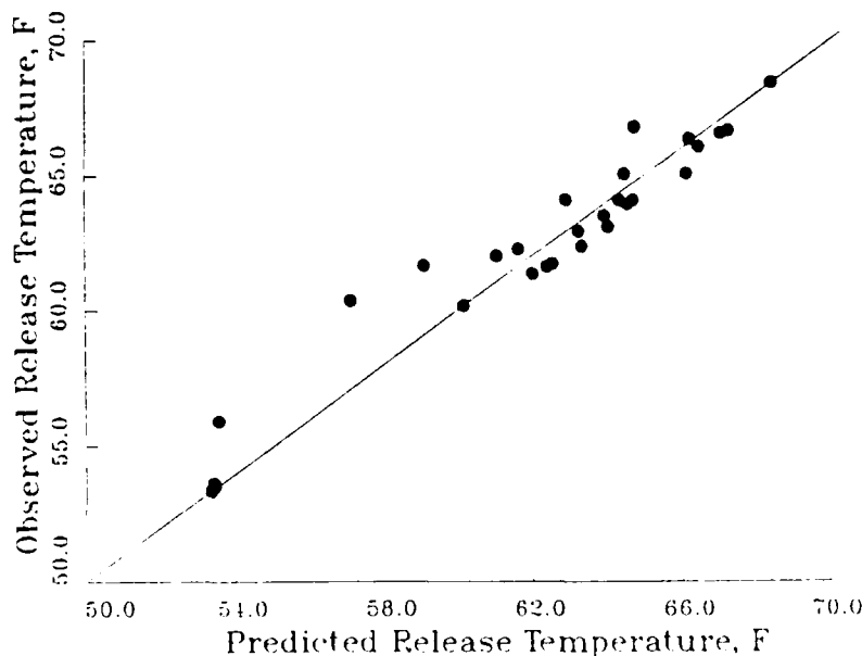
Figure 3. Predicted and observed release water temperatures during multi-port operations at Warm Springs Dam
