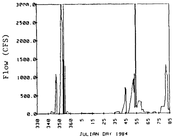
Figure 24, Discharge from Connecting Channel Gates in 1983-84 Winter
