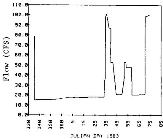
Figure 20, Discharge from Connecting Channel Gates in 1982-83 Winter
