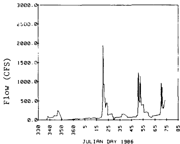
Figure 47, Discharge from Connecting Channel Gate in 1985-86 Winter
