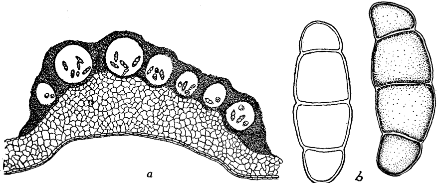
FIGURE 2.— Pauhia sideroxyli on Sideroxylon rhyncospermum (Lyon no. 61): a , section of a stroma showing locules; b , spores.
