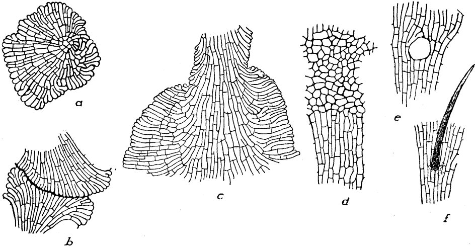
FIGURE 17.— Trichopeltis reptans : a , a circular thallus with no development of bands; b , (No. 637) on Vaccinium reticulatum , showing how lobes of two thalli react on contact with each other; c , showing (on specimen No. 1054) a simple band that is changing to the type with lateral development; d , (No. 1054) on Straussia sp.—a thallus in which the growth habit suddenly changed from the parallel, regular cell arrangement to an irregular arrangement; e , (No. 637) on Vaccinium reticulatum , showing how the thallus grows around a circular trichome; f , (No. 251) a thallus with the setum of another species of fungus growing through it.
