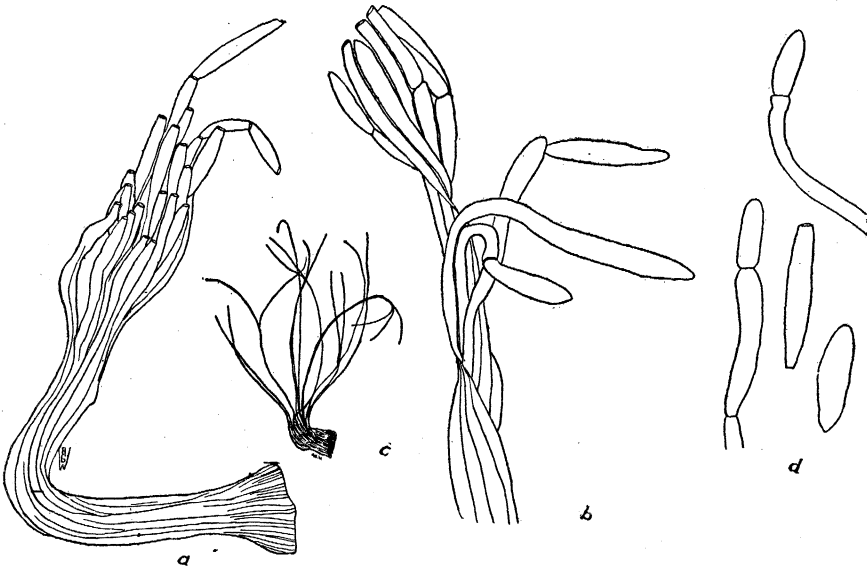
FIGURE 35.—Coremia of Graphium dubautiae (No. 650) on Dubautia laxa ; a, b, d, detail of the conidiophore apex and the conidia; c, habit sketch of a coremium.
