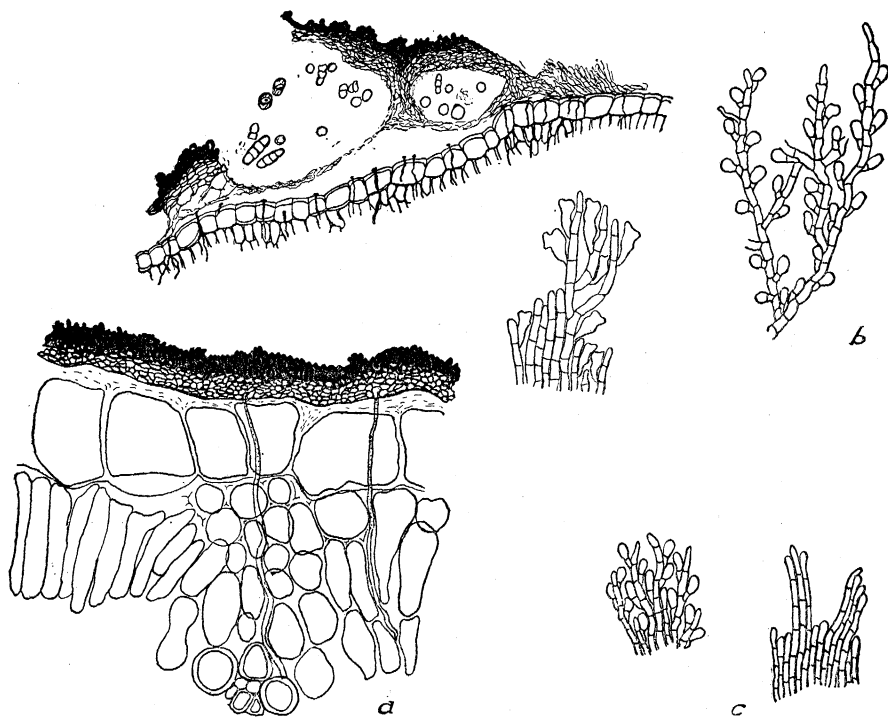
FIGURE 11.—Meliolineae: a , Actinodothis perrottetiae (No. 717) on Perrottetia sandwicensis —the mycelium at the edge, also a stroma on a leaf, showing several locules and numerous places of cuticular penetration, and the mycelium within the mesophyll; b , Amazonia ohianus (No. 842) on Metrosideros polymorpha , showing mycelium and hyphopodia; c , Actinodothis suttoniae (No. 143) on Suttonia lessertiana , showing the mycelium at the edge of a colony, a portion without hyphopodia, and another portion with atypical hyphopodia.
