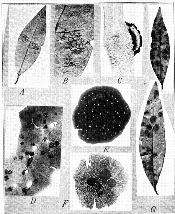
A, AULACOSTROMA OSMANTHI (NO. 136) ON OSMANTHUS SANDWICENSIS , SHOWING THE CONFLUENT CHARACTER OF THE FUNGUS; B, SAME AS A, MUCH ENLARGED; C, AULACOSTROMA OSMANTHI , CROSS SECTION OF THE PERITHECIA SHOWING THE CHARACTER AND ARRANGEMENT OF THE ASCI AND OF THE PERITHECIAL COVERING; D, ECHINODES PISONIAE (NO. 651) ON PISONIA UMBELLIFERA , SHOWING THE LARGE COLONIES SCATTERED OVER THE LEAF SURFACE; E, PLURIPORUS GOULDIAE (NO. 455) ON GOULDIA CORIACEA , SHOWING NUMEROUS OSTIOLES; F, THALLUS OF SEYNESIOPELTIS TETRAPLASANDRAE , SHOWING SEVERAL PERITHECIA; G, CALOTHYRIELLA OSMANTHI (NO. 135) ON OSMANTHUS SANDWICENSIS , SHOWING THE COLONIES ON THE LEAVES.
