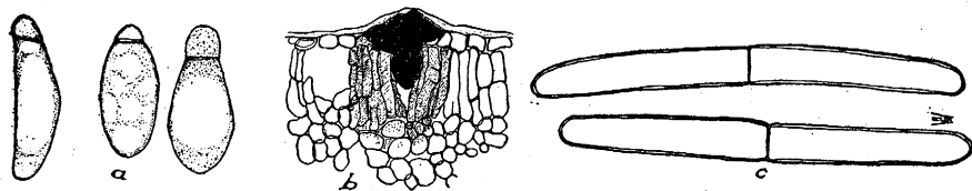
FIGURE 6.— a , Apiospora montagnei —ascospores; b , Oligostroma suttoniae (No. 868a) on Suttonia lessertiana —spores and young stroma below the cuticle and extending between the palisade cells; c , Oligostroma suttoniae —spores.
