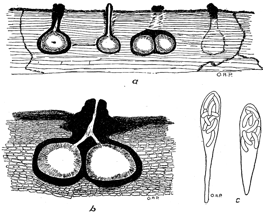
FIGURE 25.— Lageniforma bambusae on Bambusa : a, diagrammatic section of bamboo showing formation of perithecia deep within the host tissue, with a long rostrum reaching to the surface, an indistinct clypeate covering, and dark lines bounding the affected region; b, section of two perithecia having a common rostrum, showing the thick perithecial wall and the large hymenial region; c, asci.
