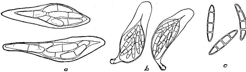
FIGURE 27.—Asci and spores: a, of Mycosphaerella freycinetiae (Forbes no. 3) on Freycinetia arnotti ; b, of Sphaerulina cibotii (No. 545); on Cibotium menziesii ; c, spores.
