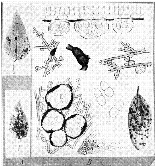
A, ECHINODELLA COCCULI (NO. 998A) ON COCCULUS FERRANDIANUS , SHOWING THE NUMEROUS SMALL COLONIES; B, LEAF OF EUPHORBIA , SHOWING THE DISTRIBUTION OF QUESTERIA EUPHORBIAE , THE GELATINOUS PERITHECIA, ASCI, SPORES, AND MYCELIUM.
