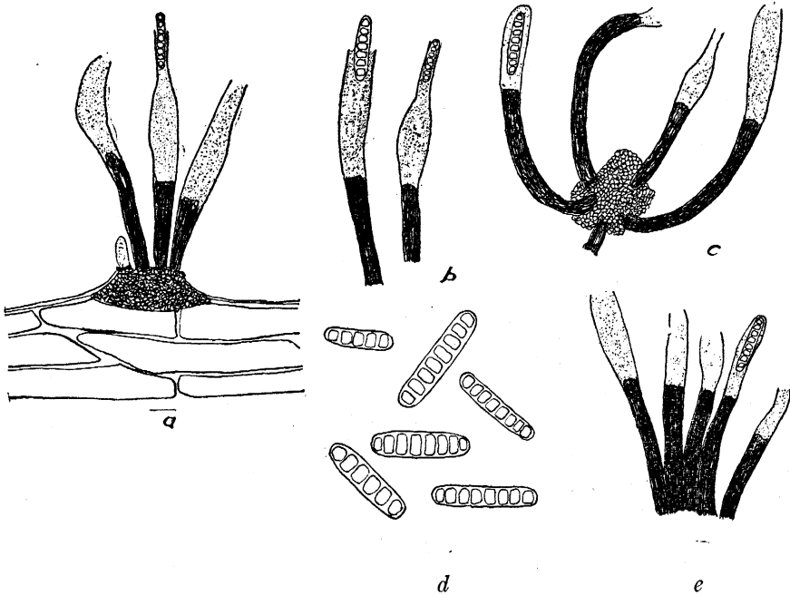
FIGURE 34.— Excioconidium cibotii (No. 810) on Cibotium chamissoi : a, showing four conidiophores arising from a small tubercular base; b, two conidiophores showing conidia emerging; c, showing conidiophores; d, conidia; e, conidiophores viewed from another aspect.
