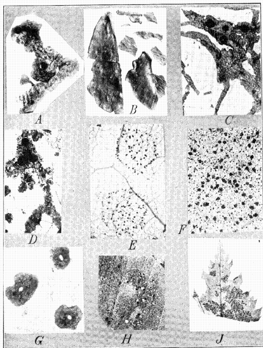
A, TRICHOPELTIS REPTANS —PHOTOMICROGRAPH OF A PORTION OF A THALLUS OF SPEGAZZINI'S SPECIMEN OF NO. 734, FUNGI CUBENSIS WRIGHTIANI; B, T. REPTANS —PHOTOGRAPH OF THE MATERIAL IN NO. 734, FUNGI CUBENSIS WRIGHTIANI; C, T. PULCHELLA —PHOTOMICROGRAPH OF PART OF SPEGAZZINI'S SPECIMEN NO. 2365; D, T. CHILENSIS —PHOTOMICROGRAPH OF SPECIMEN FROM SPEGAZZINI'S COLLECTION.—E-J, MICROTHYRIELLA , HEXAGONELLA , AND ANOMOTHALLUS : E, MICROTHYRIELLA HIBISCUS (NO. 100) ON HIBISCUS , GIVING GENERAL VIEW OF TWO CLUSTERS OF SPOTS MUCH ENLARGED; F, SAME AS E, SHOWING PERITHECIA WITH STILL GREATER ENLARGEMENT; G, THREE PERITHECIA; H, HEXAGONELLA PELEA (NO. 248) ON PELEA ROTUNDIFOLIA —THE SMALL BLACK DOTS ARE THE FRUITING THALLI; J, ANOMOTHALLUS ERRATICUS (NO. 1055) ON RUBUS HAWAIIENSIS , SHOWING HABIT ON LEAF.
