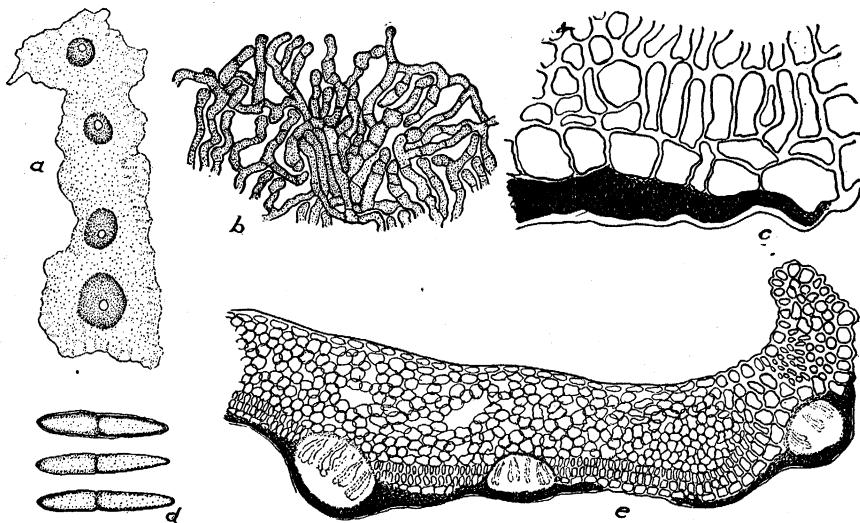
FIGURE 4.— Actinodothidopsis coprosmae (No. 457) on Coprosma : a , portion of a stroma viewed from above, showing several separate perithecia; b , mycelial structure of the edge of a stroma; c , showing position of the stroma below the cuticle; d , spores; e , the clypeate stroma and three locules.
