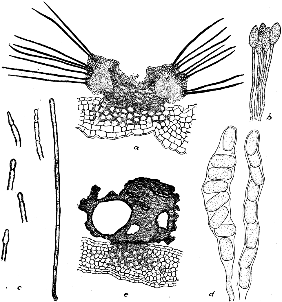
FIGURE 1.— Yoshinagella : a, microtome section of a stroma of Y. polymorpha , showing the characteristic palisade arrangement of the stroma—the hypostroma penetrates deep into the mesophyll—the origins of the setae from the rim of the stroma, the developing perithecia under the rim of the stroma, and the central cavity lined with conidiophores.—b-d, Y. polymorpha (No. 694) on Cibotium menziesii : b, conidiophores and conidia; c, setae and setal tips; d, asci with spores; e, Yoshinagella nuda on Cibotium chamissoi —section of a stroma.
