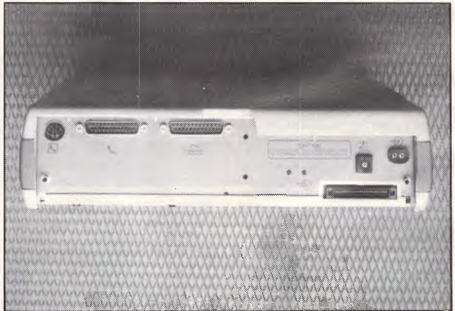
Internal modem output, two RS232s, the system expansion bus and two power inputs
