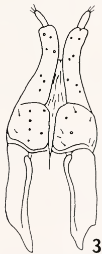
Figs. 1-3. Microcylloepus formicoideus sp. nov. 1, adult, dorsal view. 2, male genitalia. 3, female genitalia.
