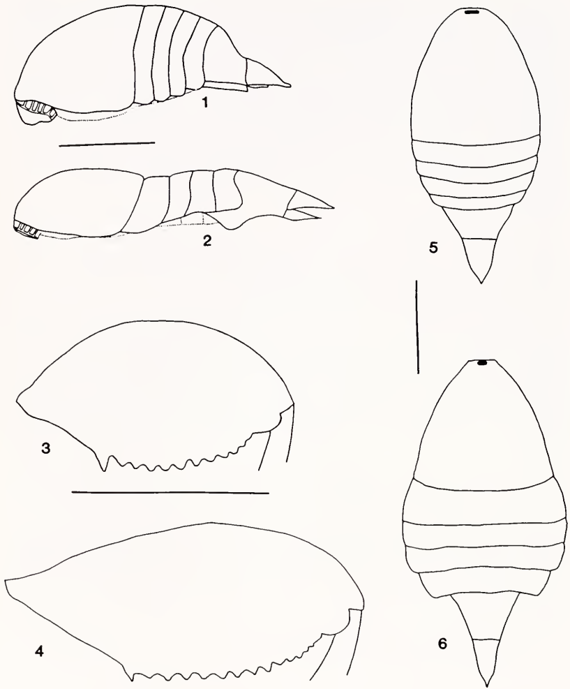
Figs. 1-6. Acanthochalcis spp. (males). A. nigricans : 1, Abdomen, lateral view; 3, Hindfemur, lateral view; 5, Abdomen, dorsal view. A. unispinosa : 2, Abdomen, lateral view; 4, Hindfemur, lateral view; 6, Abdomen, dorsal view. Scale lines 2.0 mm.
