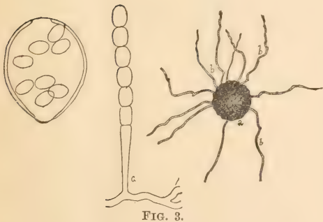
FIGURE 3. Sphaerotheca Castagnei , Lév.: a, perithecium with b appendages,—magnified 90 times; c, fertile hypha or conidiophore, bearing six conidia which readily separate at the constrictions,—magnified 190 times; d, the single ascus with eight spores,—magnified 250 times.
