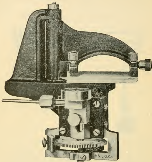
FIG. 232.—Clinic microtome with freezing attachment.
