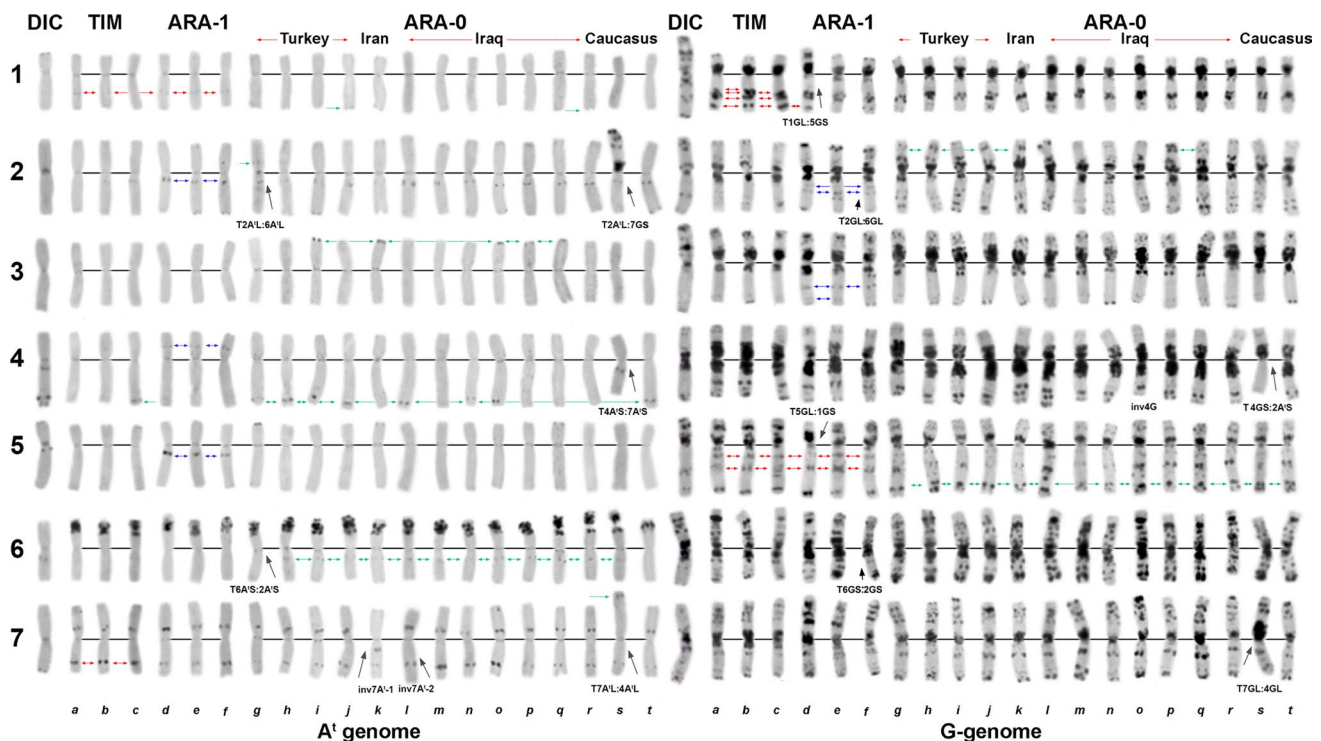
Fig. 4 Comparison of the C-banding patterns of T. dicoccoides (DIC), T. timopheevii (TIM, a – c , normal karyotypes), T. araraticum ARA-1 ( d – f ) and ARA-0 ( g – t ). DIC (IG 117174, Gaziantep), a —KU-1818 (Georgia); b —PI 119442; c —TA1900; d —IG 116165; e —PI 654340; f —KU-1950; g —Citr 17677; h —KU-8917; i —KU-8909; j —KU-1933 (all from Turkey); k —Citr 17680 (Iran); l —PI 427381 (Erbil, Iraq); m —PI 538518; n —PI 427425 (Dahuk, Iraq);
