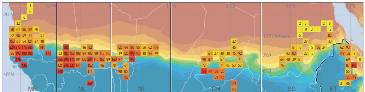
Figure S11. Density per ha of woody plants 1 m high. Average number of woody plants ( n/\text{ha} \pm \text{SD} ) in grid cells: 108 \pm 82 . Estimated overall density in Africa in the region shown on the map (10 million km 2 ; 7–22°N, 17°W–42°E): 87 per ha, based on averages given in the table for 11 rainfall zones and 6 longitudinal bands; interpolated values are marked grey. Estimated total number of woody plants in the same region: 87 billion, of which 10 billion is interpolated; range 80–94 billion (split-half).
