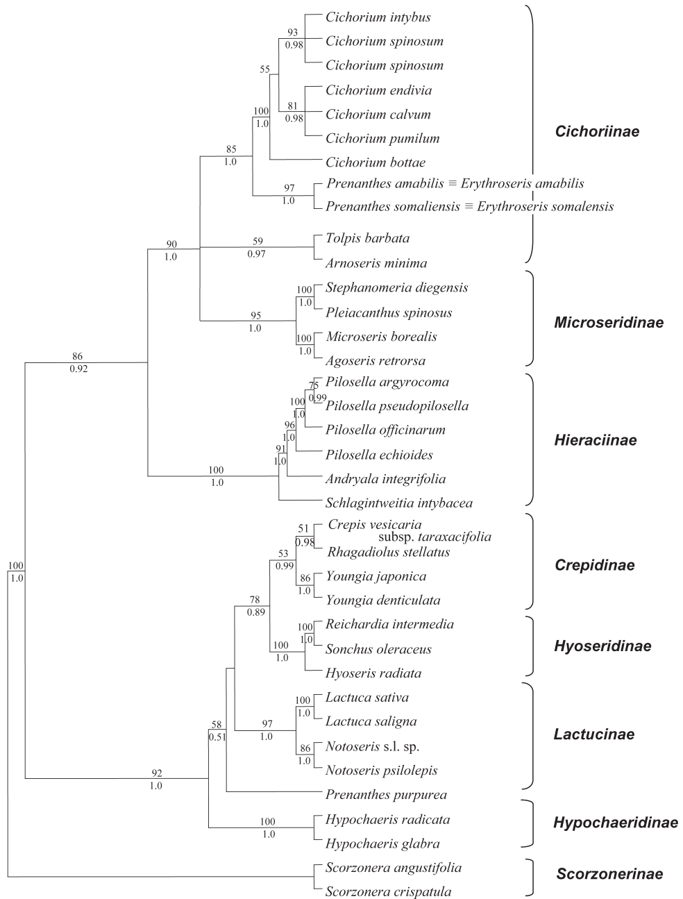
Fig. 1. Strict consensus tree of the two most parsimonious trees of the rDNA ITS analysis. Bootstrap percentages greater than 50 are given above the branches and posterior probabilities above 0.50 are depicted below.
