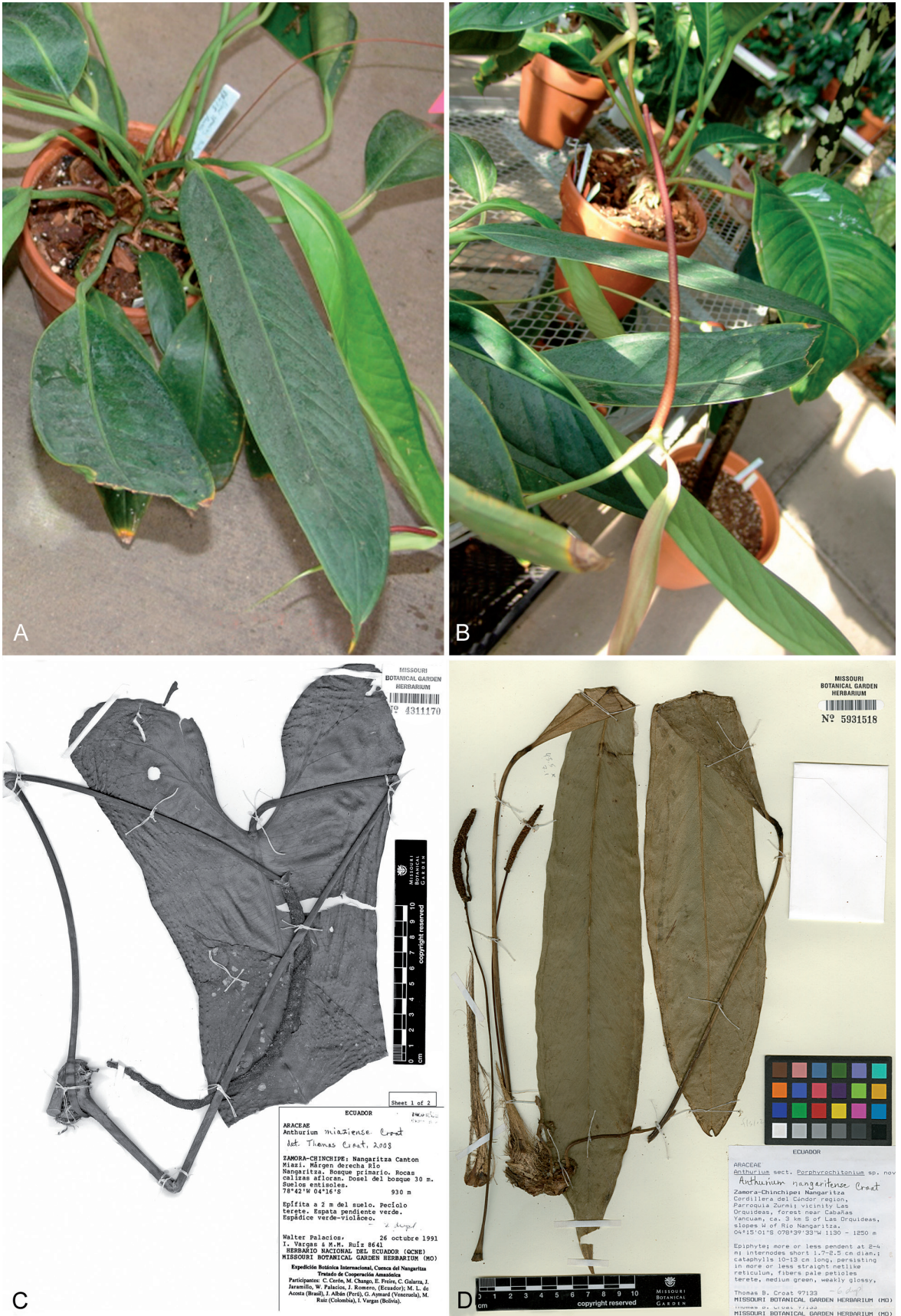
Fig. 2. A–B: Anthurium collettianum – habit of potted plant, petioles, cataphylls and inflorescence, Croat 87475 (A), inflorescence (B); C: A. miazense – holotype specimen at MO, Palacios & al. 8641; D: A. nangaritense – holotype specimen at MO, Croat 97133.
