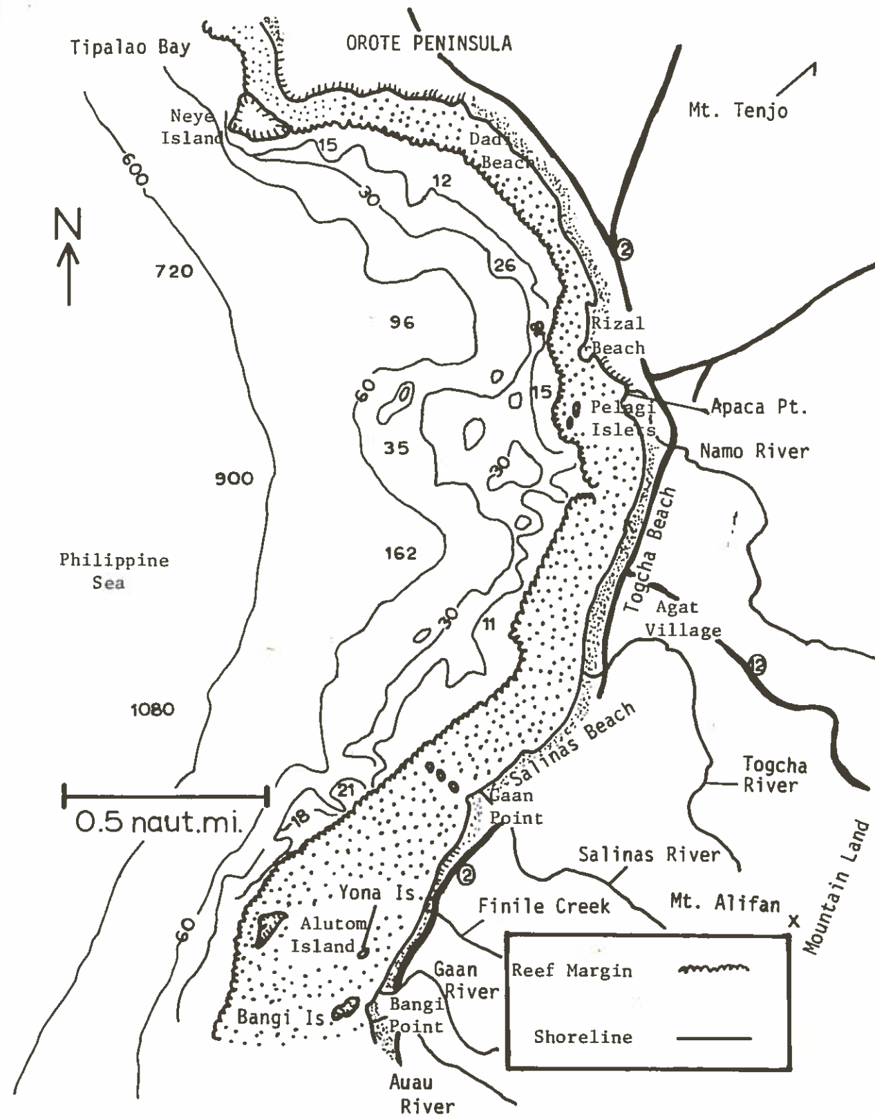
Fig. 2. General location map for the Agat Bay study area. Submarine contour depths are given in meters and the reef flat platform is stippled.
