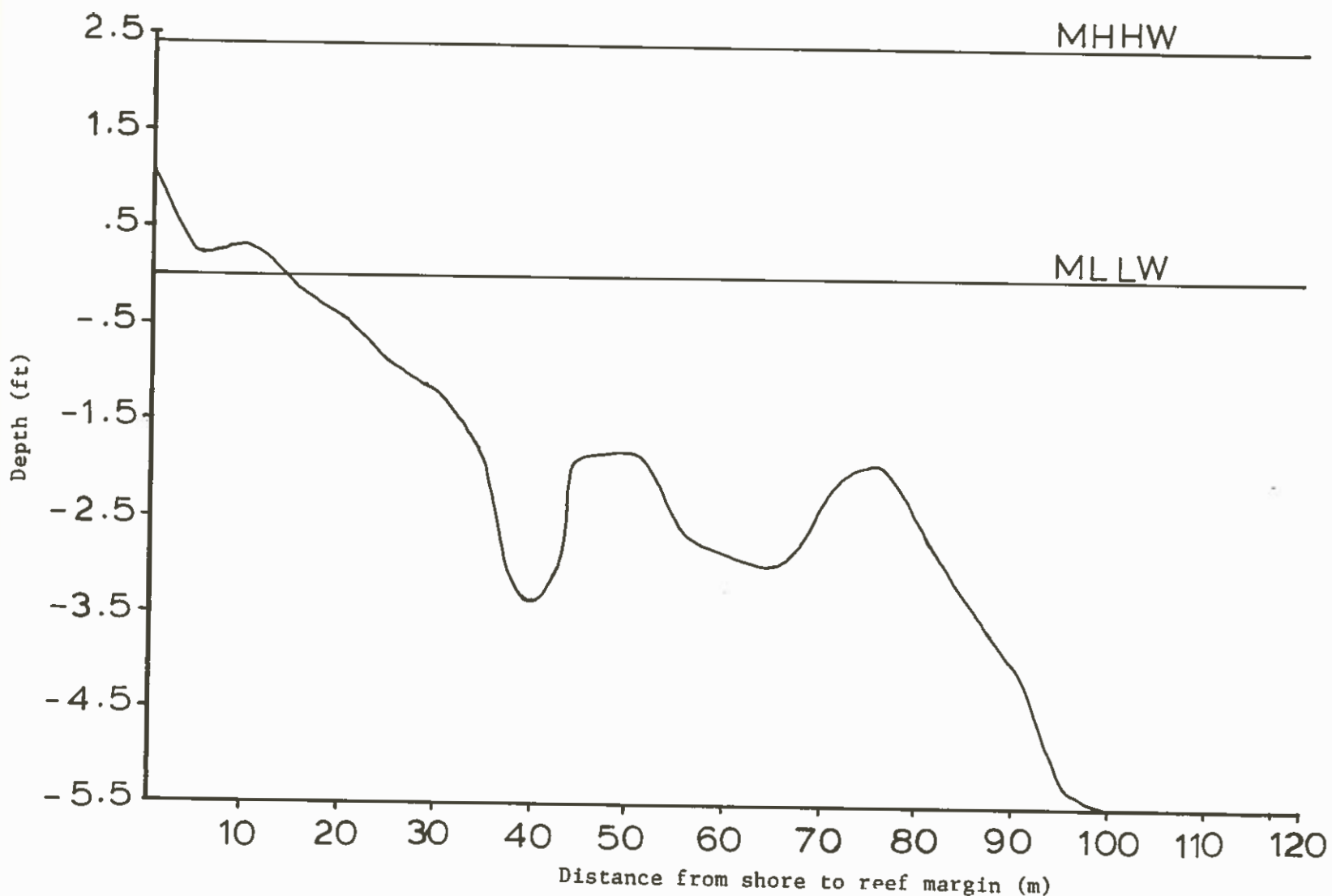
Fig. 20. Shows a vertical profile transect taken at Station 6. Profile is shown in relation to the MLLW and MHHW.
