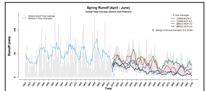
Figure 7.4: Spring Runoff (April–June). Spring runoff showed a steady decline during the recent drought period (9.3). The recent drought is shown in blue line, at the end of the current record, and four modeled future climates are portrayed in colored lines on the right.
