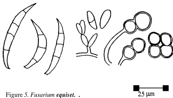
Figure 5. Fusarium equiseti .
