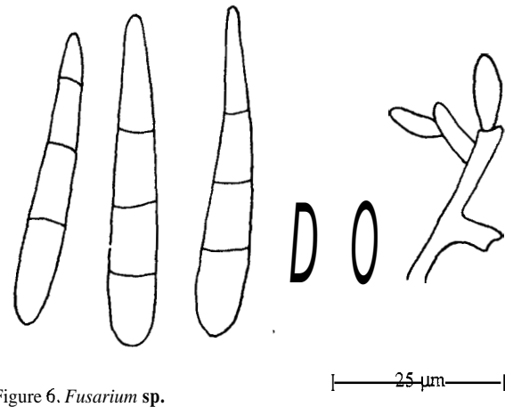
Figure 6. Fusarium sp.
