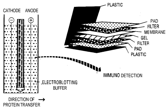
Figure 9. Western immunoblot
