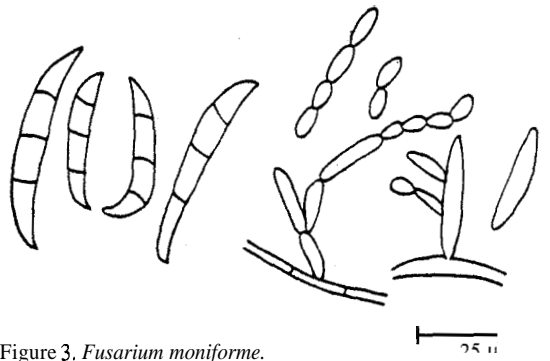
Figure 3. Fusarium moniforme .
