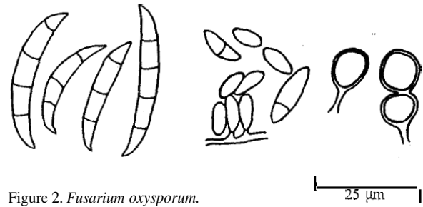
Figure 2. Fusarium oxysporum .
