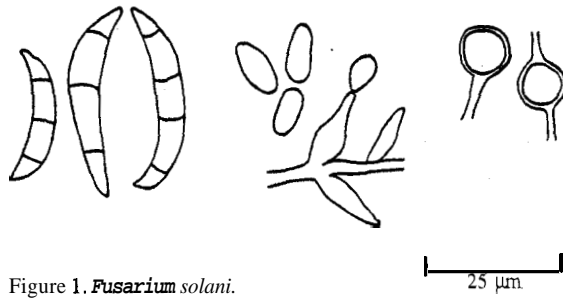
Figure 1. Fusarium solani .
