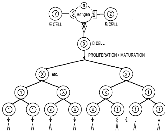
Figure 6. Clonal selection
