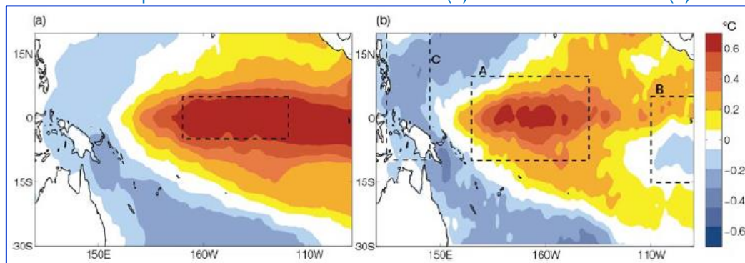
Sea surface temperature anomalies associated with (a) Canonical El Niño and (b) El Niño Modoki
