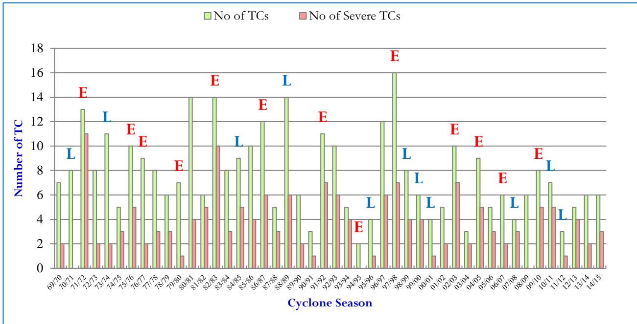
Figure 4.7: Number of TC in the Southwest Pacific during El Nino & La Nina Years.
