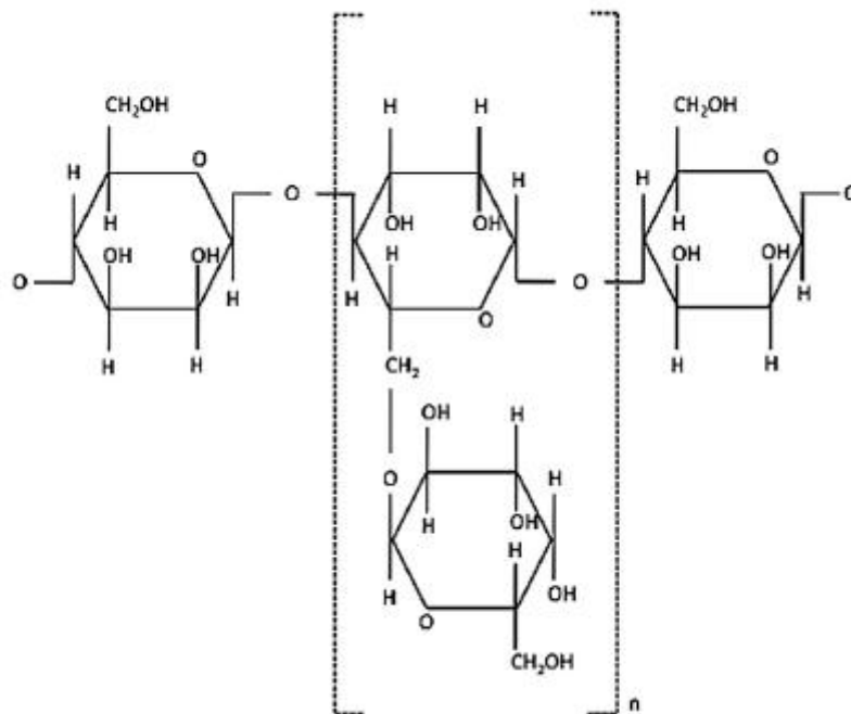
Figure 16: General molecular structure of galactomannan (Cerqueira, Souza et al. 2011).
