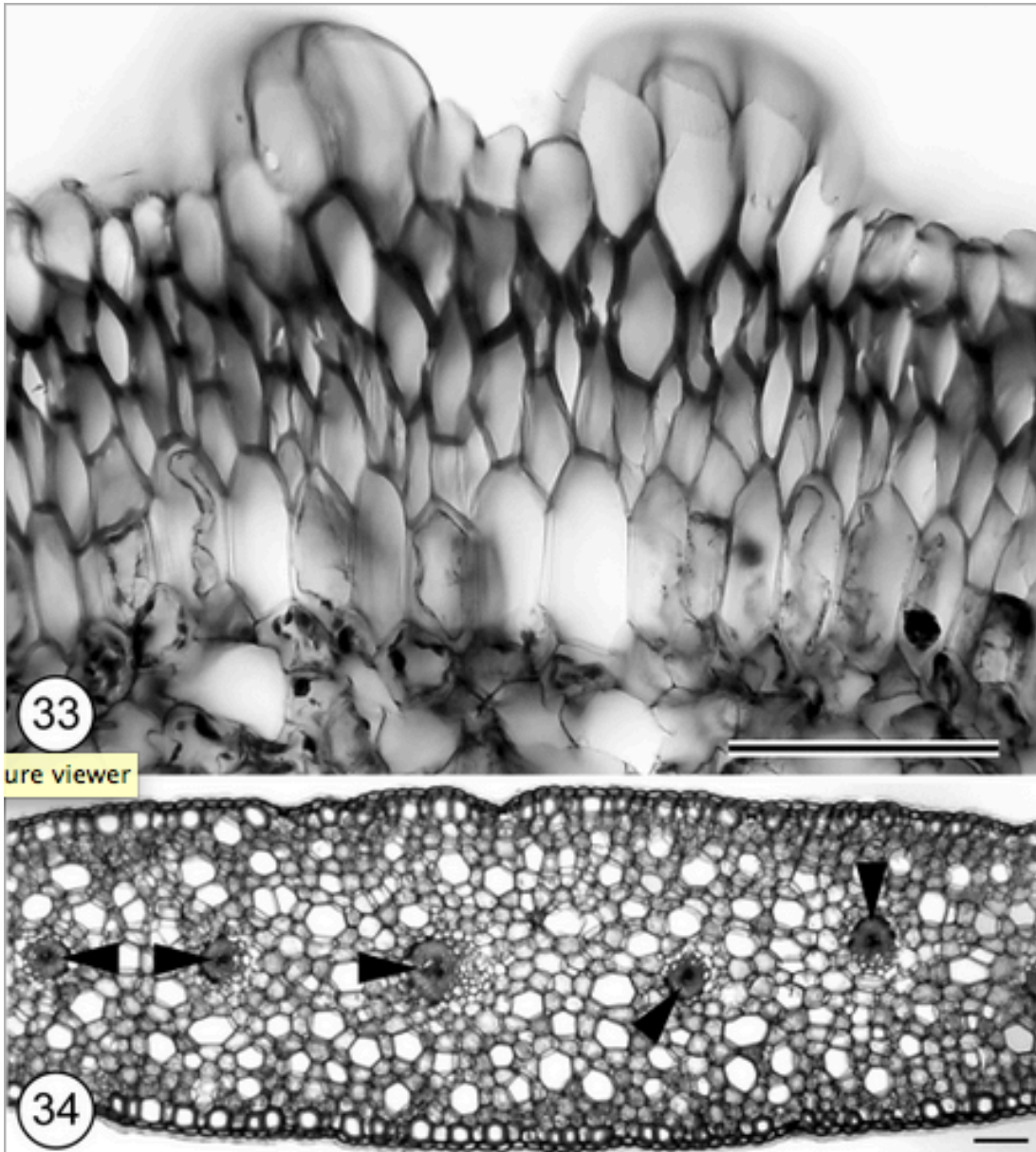
Figure 33–34. Fig. 33. Root TS of Tridactyle crassifolia showing tufts in epivelamen. Scale bar = 100 \mu\text{m} . Fig. 34. Leaf TS of Ypsilopus viridiflorus showing twisted vascular bundles (phloem poles indicated by arrowheads). Scale bar = 200 \mu\text{m} .
