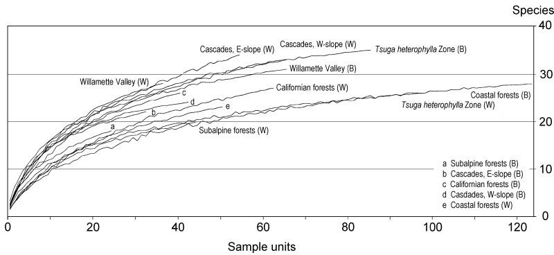
Fig. 15. Number of calicioid species as function of sample size in field specimens of conifer bark (B) and conifer wood (W) from the different forest zones.
