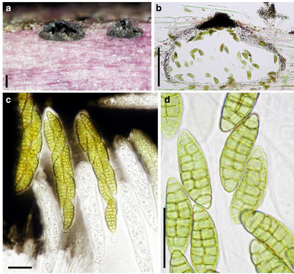
Fig. 64 Murispora rubicunda (from IFRD 2017). a Habitat section of the immersed ascómata. b Section of an ascoma. Note the thin peridium and cells of textura angularis . c Mature and immature asci. d Muriform ascospores. Scale bars: a , b = 100 \mu\text{m} , c , d =20 \mu\text{m}
