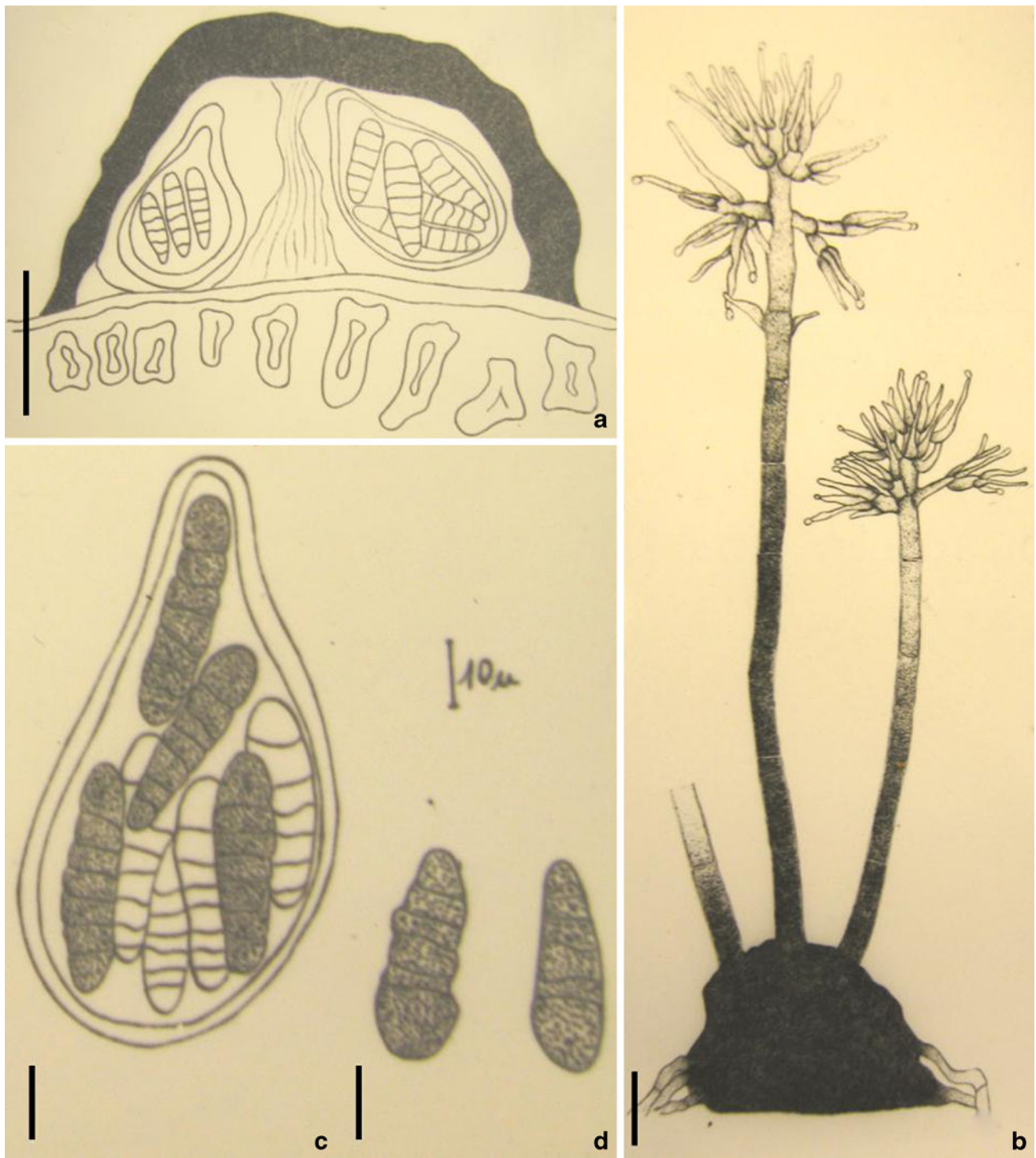
Fig. 102 Kriegeriella mirabilis (from S reg. nr F12638, isolecto- type ). a Section of a superficial ascoma. b Anamorphic stage. c Obpyriform ascus. Note the pigmented ascospores and hyaline ascospores coexisted in a single ascus. d Ascospores. Scale bars: a =
