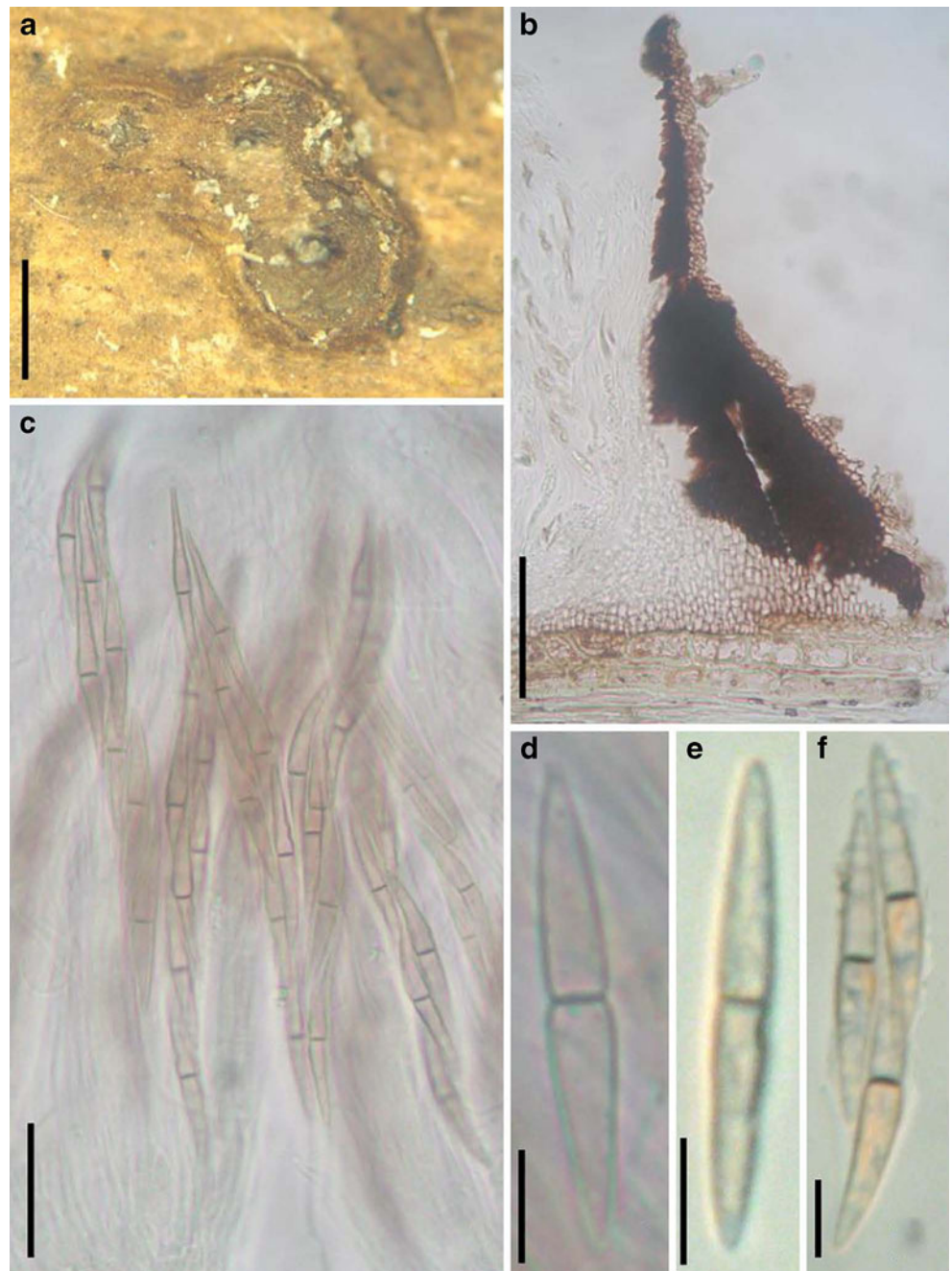
Fig. 8 Astrosphaeriella fusispora (BISH 145726). a Ascocmata forming a small group on host surface. Note the remains of the host forming flanges around the ascocmata. b Section of the partial peridium. Note the black peridium and wedge of palisade cells between the lateral and basal walls. c Asci in trabeculate pseudoparaphyses. d–f Narrowly fusoid ascospores. Scale bars: a =1 mm, b =100 \mu m, c =50 \mu m, d =15 \mu m, f =10 \mu m
