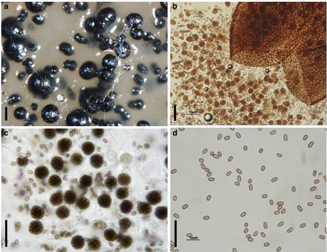
Fig. 99 Pycnidophora dispersa (a from CBS 297.56; b–d from MSC 133.118, type). a Ascomata scattering on the surface of the substrate. b Crashed ascoma. Note the numerous released asci. c Globose asci
