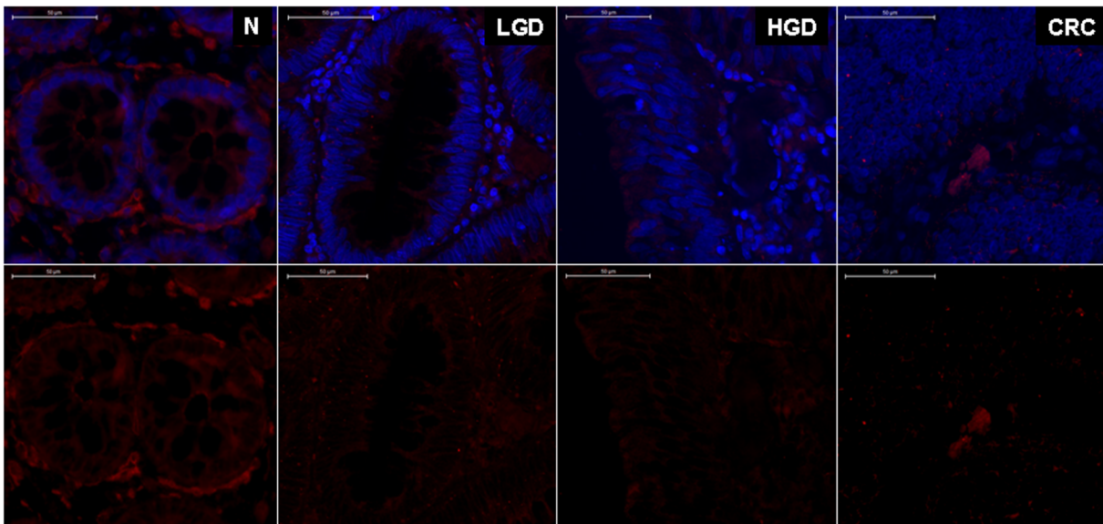
Fig 3. A. Gene expression of SFRP1 during ACS measured by mRNA expression microarray analysis. As indicated, transcript levels decreased across in LGD, HGD and CRC samples in 3 out of 4 SFRP1 transcripts. B. Protein expression of SFRP1 protein measured by immunohistochemistry. SFRP1 protein expression gradually decreased during ACS. The epithelial SFRP1 expression showed a continuous decrease during ACS. Epithelial SFRP1 expression was decreased in LGD compared to normal epithelium, but stromal SFRP1 protein expression was retained. In HGD and CRC samples, both epithelial and stromal SFRP1 protein expression was significantly reduced. Red staining: SFRP1 , blue staining: Hoechst nuclear staining. N: normal sample, LGD: low-grade dysplasia, HGD: high-grade dysplasia, CRC: colorectal cancer
