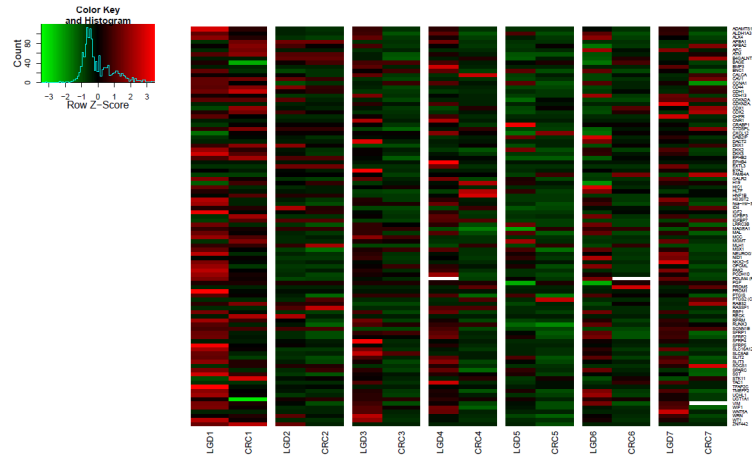
Fig 1. DNA methylation heatmap for synchronous LGD and CRC samples from the same patient. The number of hypermethylated genes and methylation levels were higher in LGD than in synchronous CRC.
