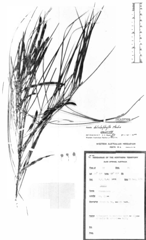
Fig. 3. Acacia dolichophylla sp. nov. (P. K. Latz 6606, holotype—PERTH).
