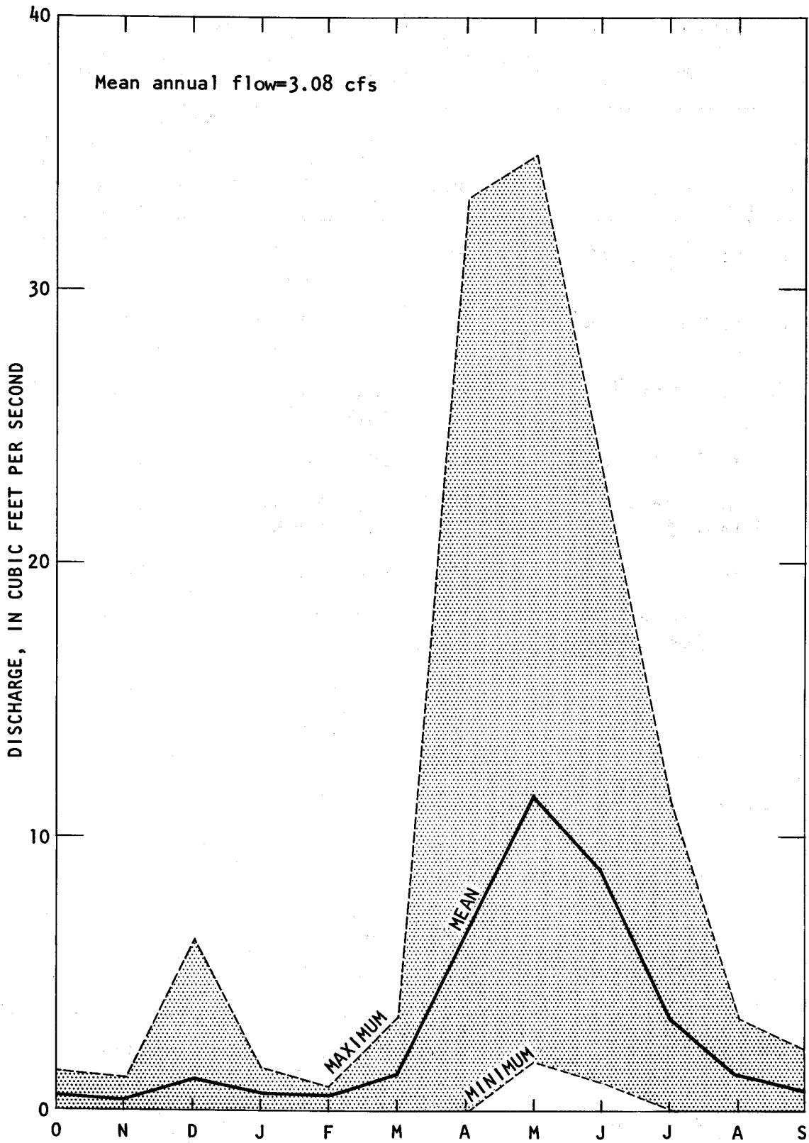
Figure 2.--Monthly flow distribution for Little Carrant Creek, water years 1965-72 (location 11/59-5ba).
