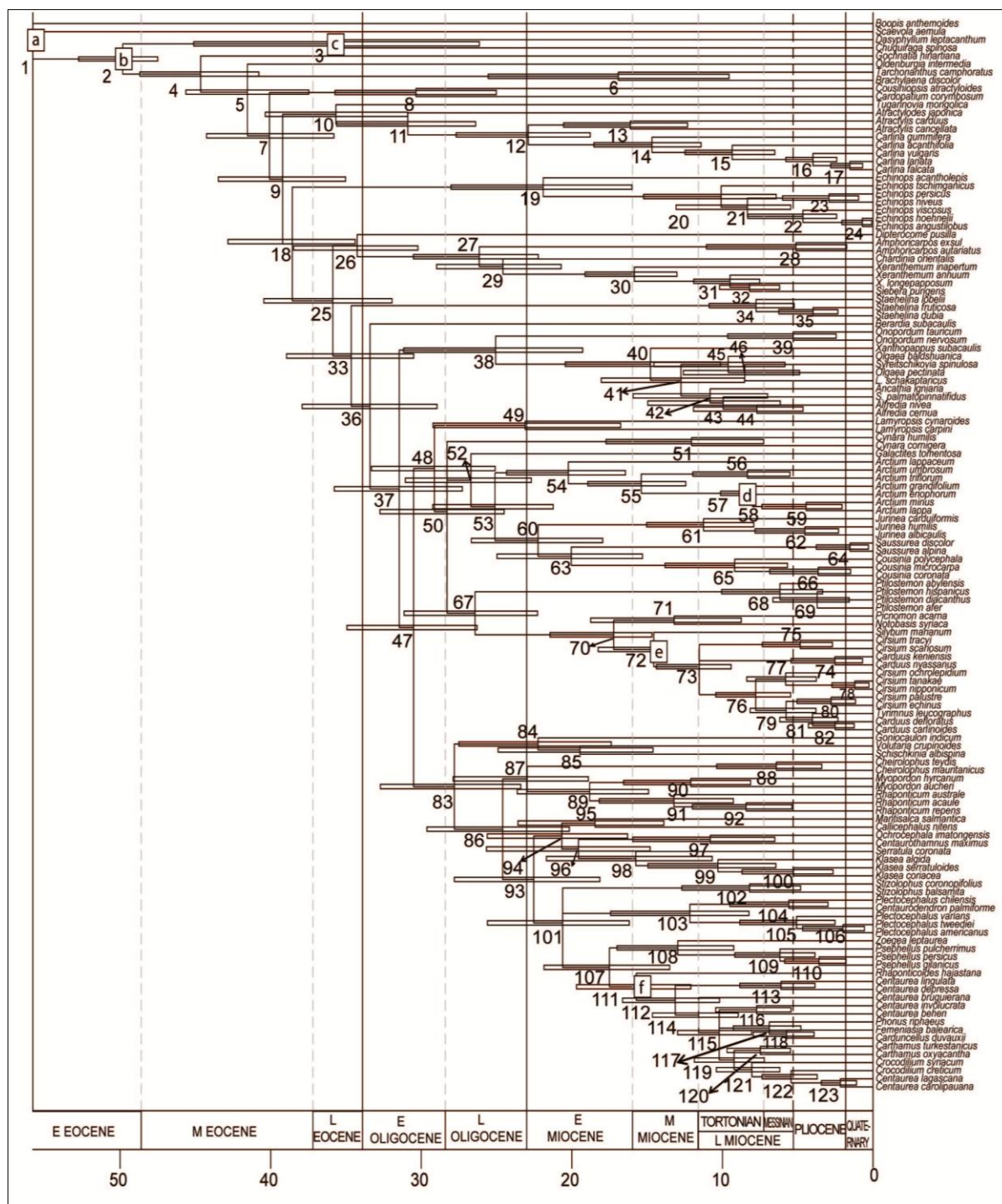
Fig. 3. Chronogram showing the majority-rule “halfcompat” consensus tree from the Bayesian analysis of the chloroplast dataset of tribe Cardueae ( Compositae ) and close allies, with mean divergence times and confidence intervals (95%) for nodal ages estimated by penalized Likelihood (PL) over a sample of 1000 trees from the MCMC stationary distribution of this analysis. Lower case letters in box indicate the nodes calibrated with fossil constraints. Node numbers refer to Appendix S3 (see Supplemental Data with the online version of this article).
