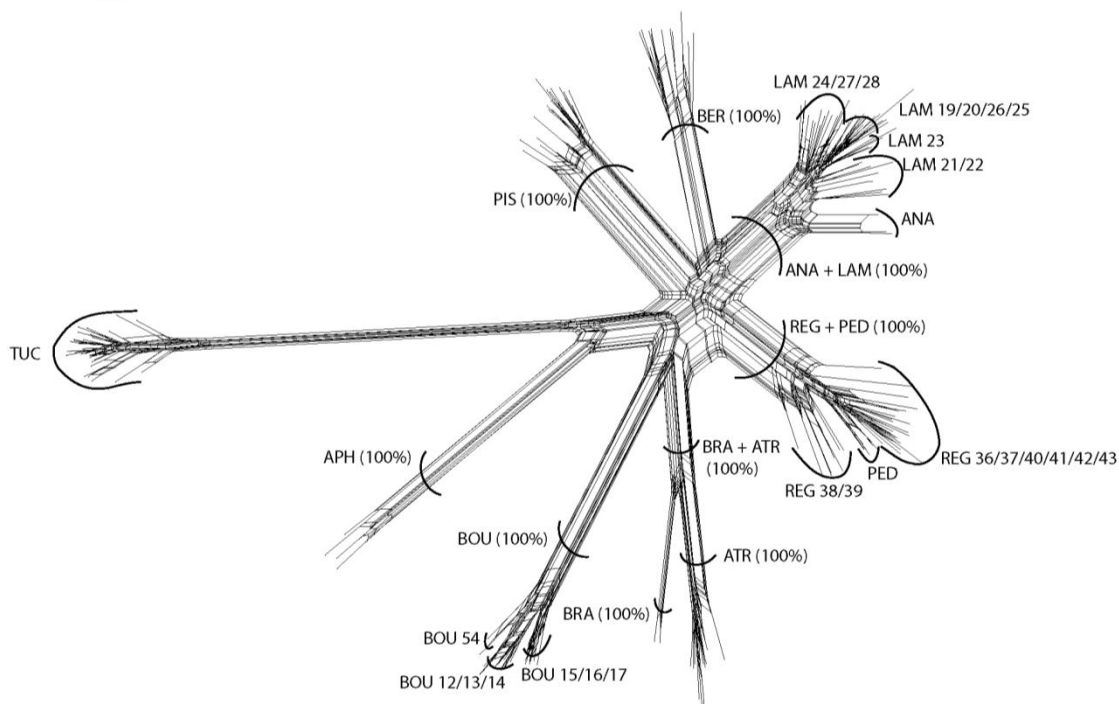
Fig. 3. Plot of the Principal Coordinate Analysis of 346 AFLP markers based on Dice's similarity coefficient.
