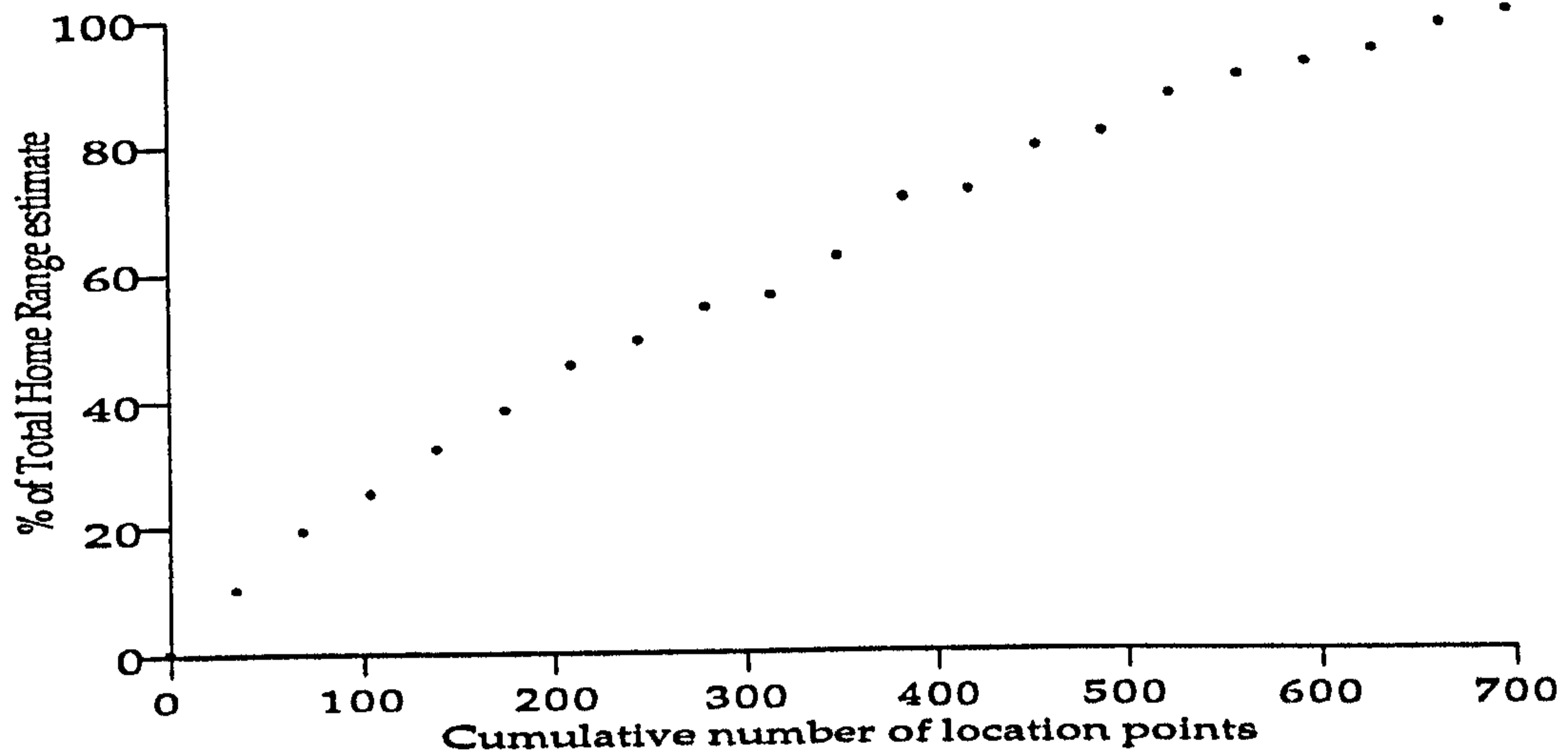
Figure 8.4.a. Group N151
