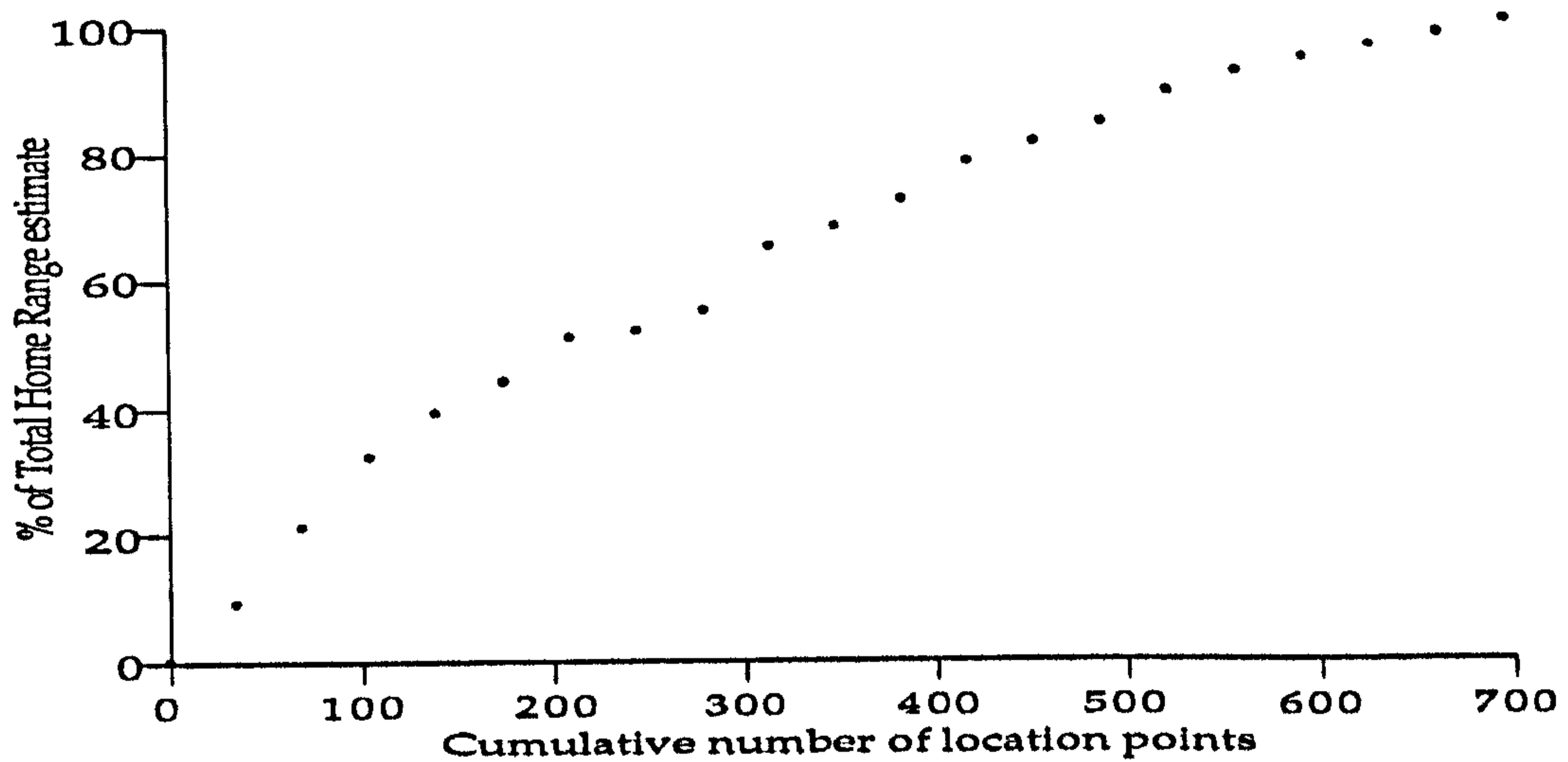
Figure 8.4.b. Group N152
