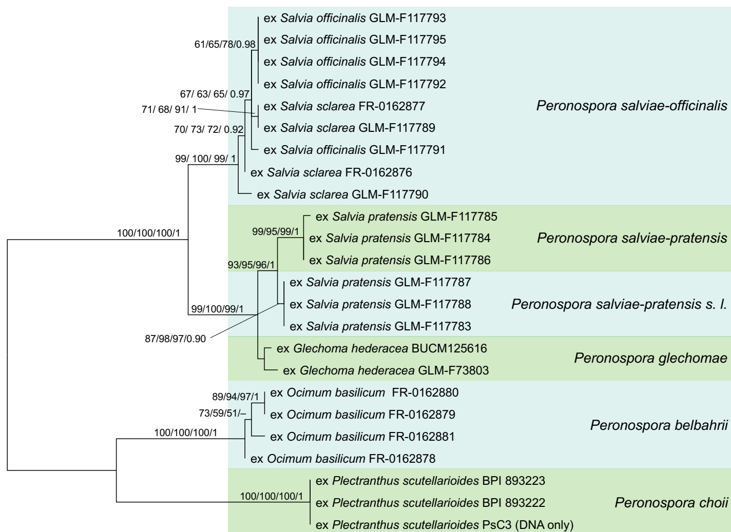
Fig. 5. Phylogenetic reconstruction in MP inferred from the concatenated alignment of six genes (ITS, ef1a , hsp90 , βtub , cox1 , cox2 ). MP, ME and ML bootstrap support values above 50 %, and a posteriori probabilities above 0.9 are given at first, second, third, and fourth positions at the branches, respectively. A minus sign denotes lacking support for the present or an alternate topology.
