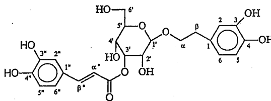
1 sanangoside
