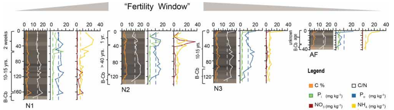
Figure 4. Fertility over time. The three different phases in the cycle of cultivation represented by fields N1 (two weeks after addition of fresh biomass to rehabilitate a field that had been left fallow for at least 10 years), N2 (one year after rehabilitation, field age > 40 years), and N3 (fallow, since about 10 years). Some fields are not only left fallow, but abandoned (AF, abandoned at least 20 years ago). Peak of chemical fertility in the layers where crop roots are concentrated is reached some months to one year after rehabilitation for cultivation (“Fertility Window”). Fertility then declines, returning to values typical of nearby uncultivated soils during the fallow period and falling even lower with abandonment. Plots show downprofile colour (visualized by conversion of spectrophotometrically measured colour space values into the RGB colour space 39 ) and chemical analysis of the main profiles (X) of fields N1, N2, and N3. Dashed lines in the background are the mean values for each chemical parameter of the topsoil (Ah) samples taken at 10 cm depth from areas near each field in the RFSA. (Graphs were plotted with Grapher and arranged using Adobe Illustrator).
