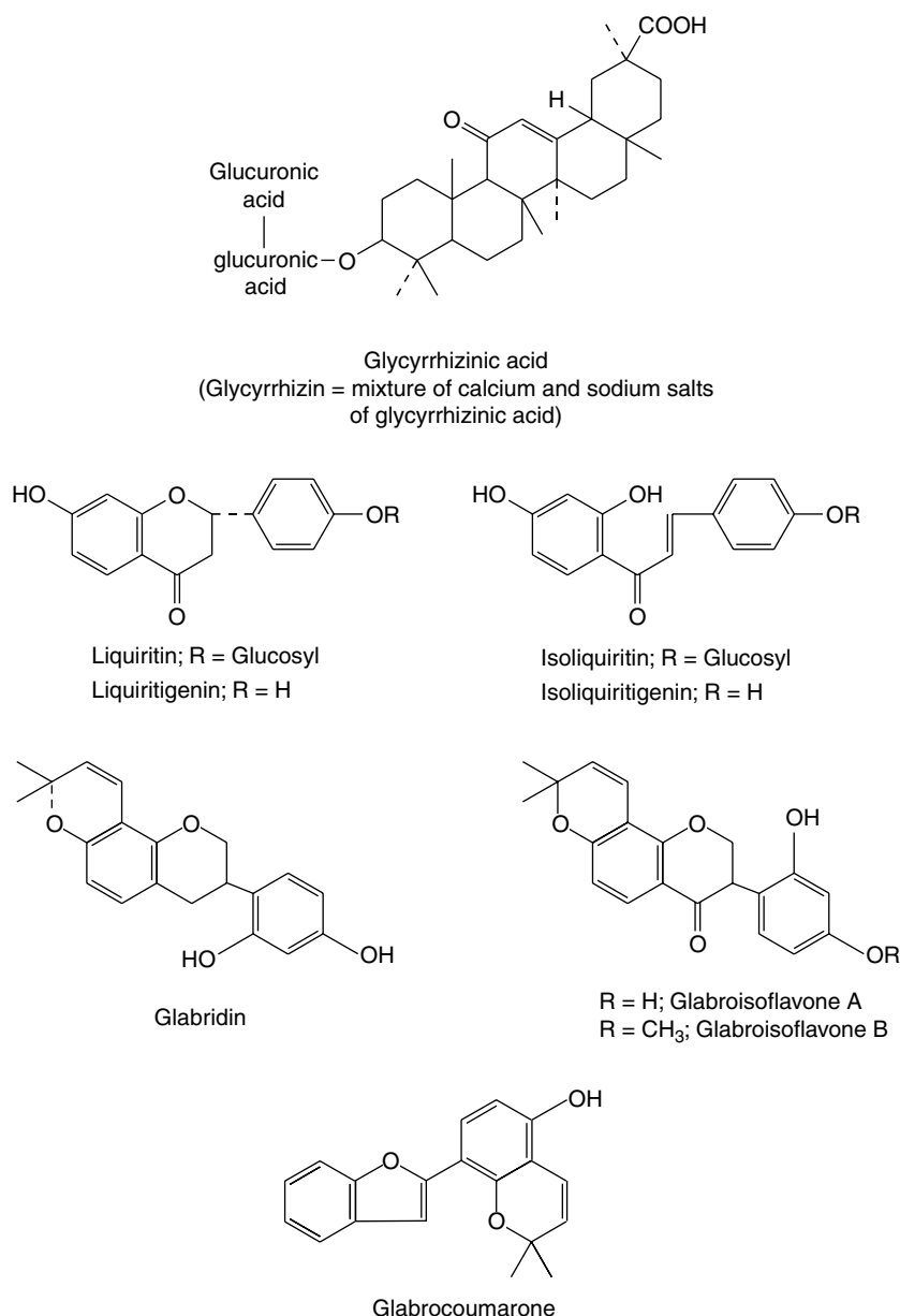
Fig. 23.12 Some constituents of liquorice root.
