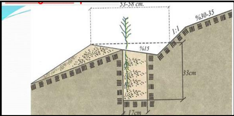
Figure 14: Gradoni-type with ditches (URL-14)
