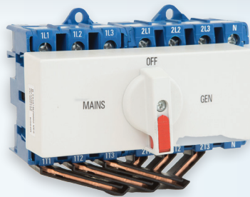
63A 3p/4p Mains-Off-Gen Din mount Shallow handle KN417
