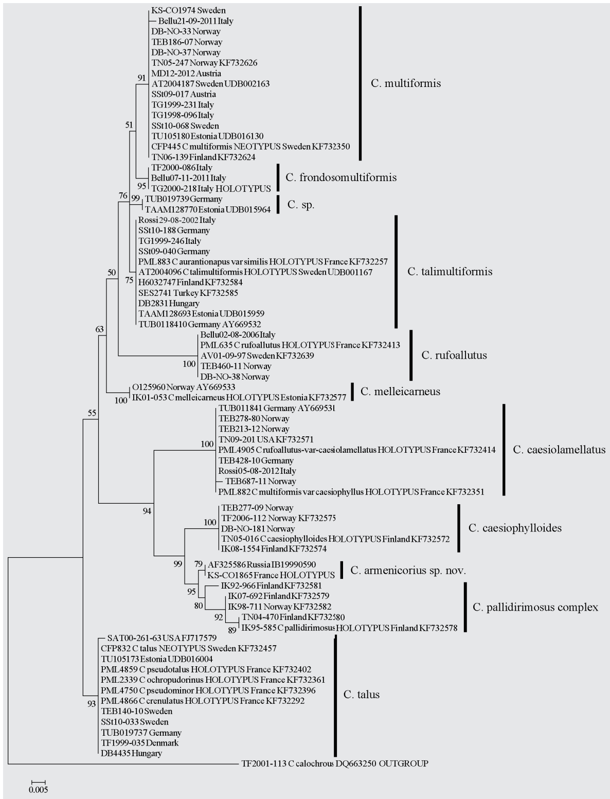
Fig. 1 – Maximum likelihood ITS phylogram of Cortinarius sect. Multifformes in Europe calculated with RAxML. Bootstrap values are given above branches. The bar indicates the number of expected substitutions per position. For each collection, herbarium number, locality (country), and GenBank/UNITE accession numbers if existed are provided.
