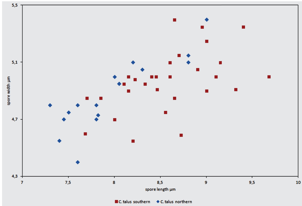
Fig. 15 – Variation in spore size of C. talus . Each symbol = MV of spore measures per basidiome. Northern = middle/northern boreal (subalpine) Betula pubescens populations. Southern = more southern Fagus-Quercus-Carpinus-Corylus-Betula pendula populations.
