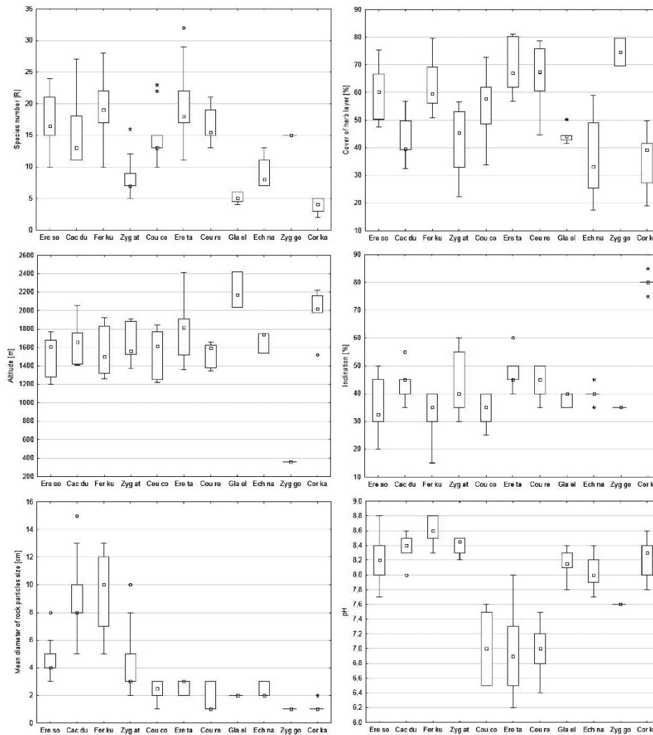
Fig. 4. Box-whisker plots of the species richness, cover of the herb layer, altitudinal distribution, inclination, pH and size of the rock particles of screens of the researched communities: Eremuretum sogdiani (Ere so), Caccinietum dubiae (Cac du), Feruletum kuhistanicae (Fer kuh), Zygophylletum atriplicoidis (Zyg at), Cousinietum corymbosae (Cou co), Eremostachyetum tadschikistanicae (Ere ta), Cousinietum refractae (Cou re), communities of Glaucium elegans (Gla el), Echinops nanus (Ech na), Zygophyllum gescharovii (Zyg go) and the Corydalidetum kashgaricae (Cor ka).
