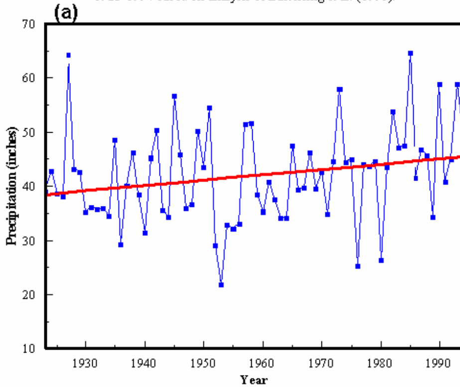
Figure Hy02. (a) Estimated mean annual precipitation amounts and (b) mean monthly precipitation amounts in the Big Piney Basin for years 1923-1994 based on analysis of Easterling et al. (1995).
