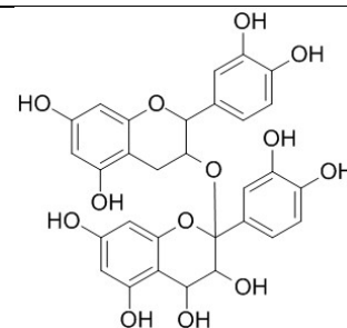
Proanthocyanidins (27)
