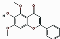
5-hydroxy-40, 7- dimethoxyflavone (40)
