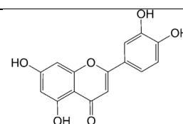
Luteolin (45)
