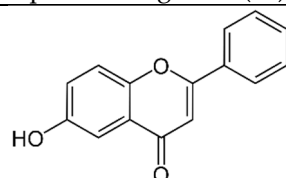
6-hydroxyflavone (29)
