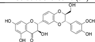
Iso bavachalcone (54)
