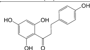
5, 7, 40-trihydroxyflavanol (22)
