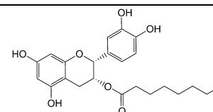
3-O-octanoyl-epicatechin (21)
