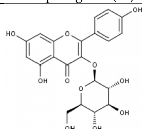
kaempferide-3-O-glucoside (50)
