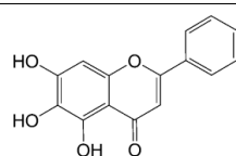
Baicalein (44)
