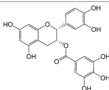
epicatechin gallate (26)
