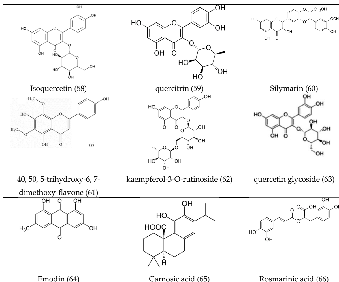
Figure 2. Chemical structures of antibacterial bioactive compounds.
