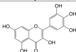
Myricetin (43)
