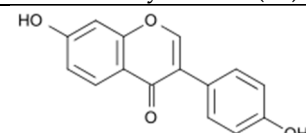
Proanthocyanidins (27)
