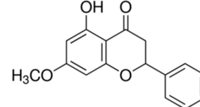
Daidzein (30)
