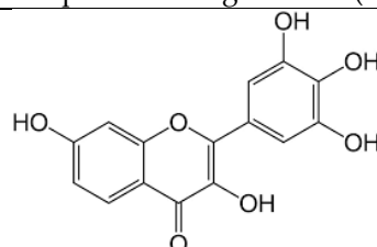
Robinetin (53)
