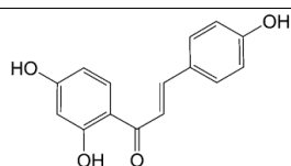
4, 20, 40-trihydroxychalcone (41)
