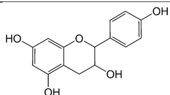
5, 7, 40-trihydroxyflavanol (22)
