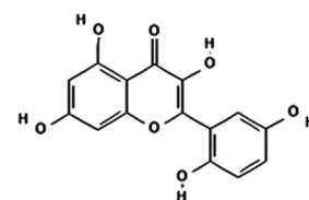
5, 6, 7, 40, 50- pentahydroxyflavone (39)
