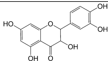
Taxifolin (38)
