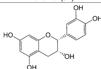
Epicatechin (35)
