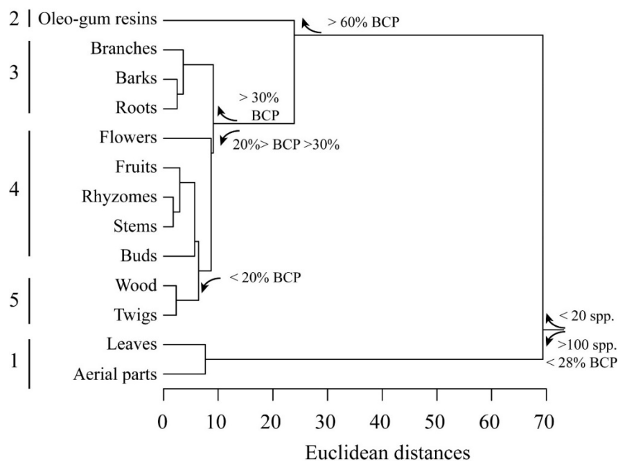
Figure 2. Cluster analysis of BCP and yield percentages according to the plant part used for extraction. Euclidean distances are calculated with average linkage method. Five clusters are evident (see text for explanation).
