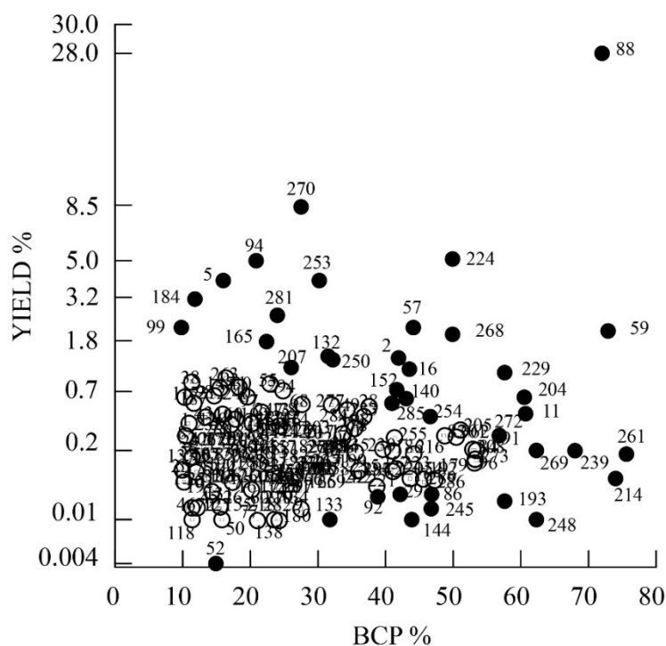
Figure 1. Scatter plot of BCP percentage vs. yield percentage. The yield axis is represented as a power of 0.3 scale in order to evidence species with yields ranging from 0.004 to 3%. Numbers correspond to plant species listed in Table 1. Filled circles outline the species outside the central group of all other species (hollow circles).
