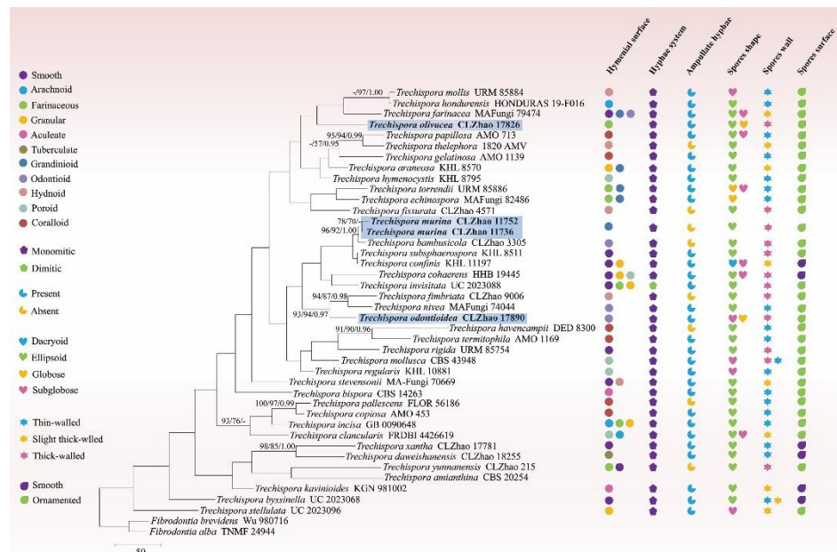
Figure 2. Maximum parsimony strict consensus tree illustrating the phylogeny of three new species and related species in Trechispora based on ITS sequences. Branches are labelled with maximum likelihood bootstrap value \geq 70\% , parsimony bootstrap value \geq 50\% , and Bayesian posterior probabilities \geq 0.95 , respectively. The new species are in bold.
