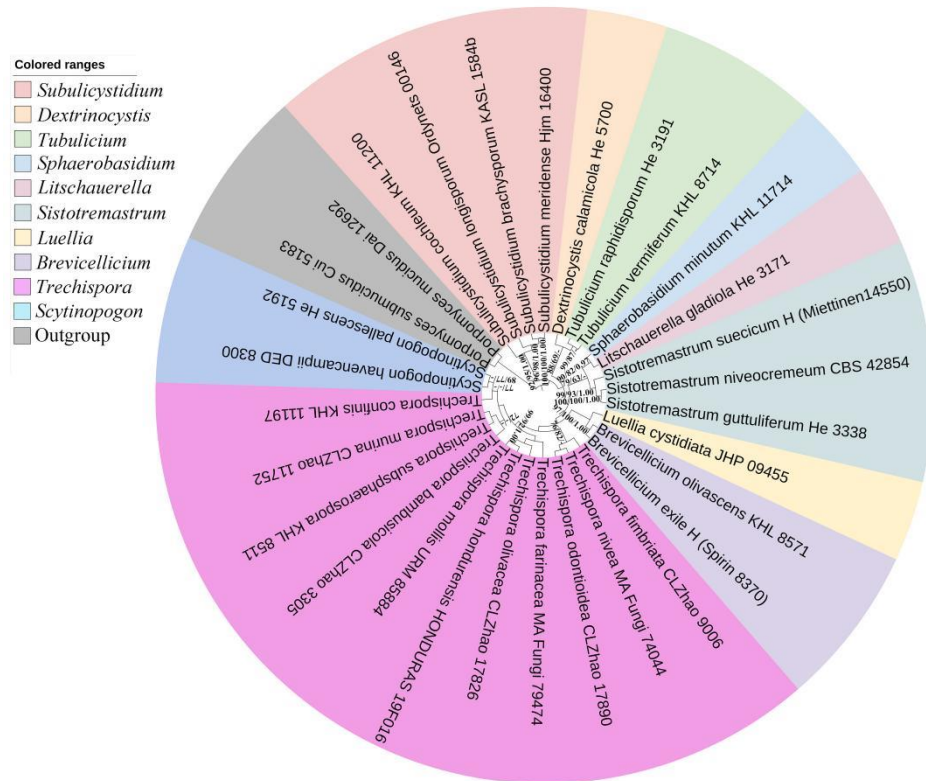
Figure 1. Maximum parsimony strict consensus tree illustrating the phylogeny of Trechispora and related genera in Trechisporales based on 5.8S+nLSU sequences. The genera represented by each color are indicated in the upper left of the phylogenetic tree. Branches are labelled with maximum likelihood bootstrap value \geq 70\% , parsimony bootstrap value \geq 50\% , and Bayesian posterior probabilities \geq 0.95 , respectively.
