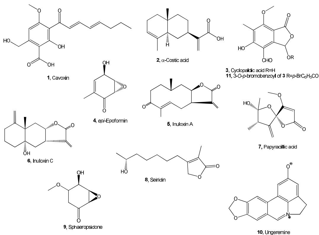
Figure 1. The structures of compounds 1–11.
