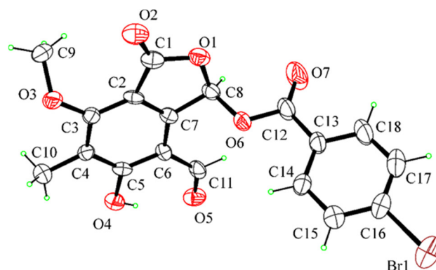
Figure 12. ORTEP view of cyclopaldic acid derivative ( 11 ) with ellipsoids drawn at the 30% probability level.
