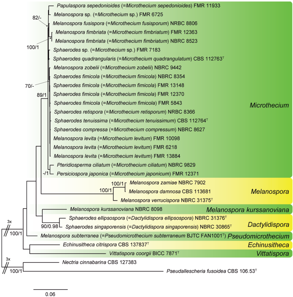
Figure 2. RAxML phylogram obtained from the combined ITS, LSU, act and tef1 sequences of our isolates and type and reference strains of the order Melanosporales. Nectria cinnabarina and Pseudallescheria fusioidea were used as outgroup. RAxML bootstrap support (BS) values above 70 % and Bayesian posterior probability scores above 0.95 are shown at the nodes. GenBank accession numbers are indicated in Table 1. Type strains of the different species are indicated with T .
