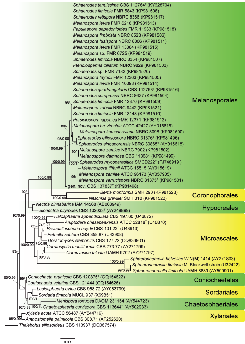
Figure 1. RAxML phylogram obtained from SSU sequences of isolates and type and reference strains included in the Melanosporales, and strains belonging to the orders Chaetosphaeriales, Coniochaetales, Coronophorales, Hypocreales, Microascales, Sordariales and Xylariales. Thelebolus ellipsoideus was used as outgroup. RAxML bootstrap support (BS) values above 70 % and Bayesian posterior probability scores above 0.95 are shown at the nodes. Type strains of the different species are indicated with T .
