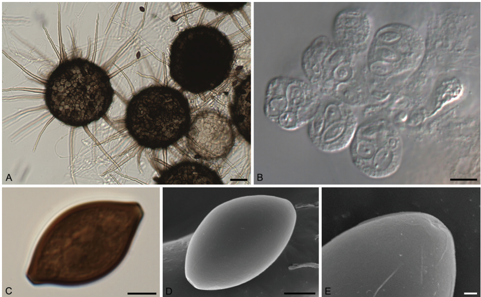
Figure 3. Echinusithecra citrispora (CBS 137837 T ). A Ascomata B Asci C, D Ascospores E Depressed germ pore. Scale bars: 50 \mu\text{m} ( A ); 10 \mu\text{m} ( B ); 5 \mu\text{m} ( C, D ); 1 \mu\text{m} ( E ).
