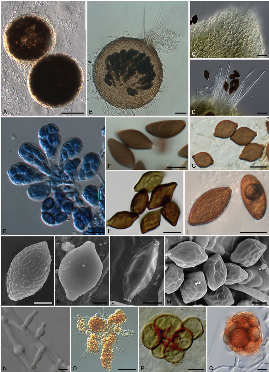
Figure 5. Morphological features of the genus Microthecium . Microthecium levitum (FMR 10098). A Non-ostiolate ascoma E Asci G Ascospores K Ascospore (SEM). Microthecium fayodii (FMR 12363). B Ostiolate ascomata F Ascospores O Variable shaped bulbils. Microthecium fimicola (FMR 5483). C Detail of cellular neck M Ascospores (SEM) P Bulbil. Microthecium quadrangulatum (CBS 112763 1 ). D Crown of setae around the ostiole L Ascospore SEM. Microthecium retisporum (NBRC 8366). H Ascospores N Asexual morph. Microthecium japonicum (FMR 12371) I Ascospores J Ascospore SEM. Microthecium sepedonioides (FMR 11933) Q Bulbil. Scale bars: 50 \mu\text{m} ( A, B, O ); 20 \mu\text{m} ( C, D ); 10 \mu\text{m} ( E–I, P, Q ); 5 \mu\text{m} ( J, L–N ); 2.5 \mu\text{m} ( K ).
