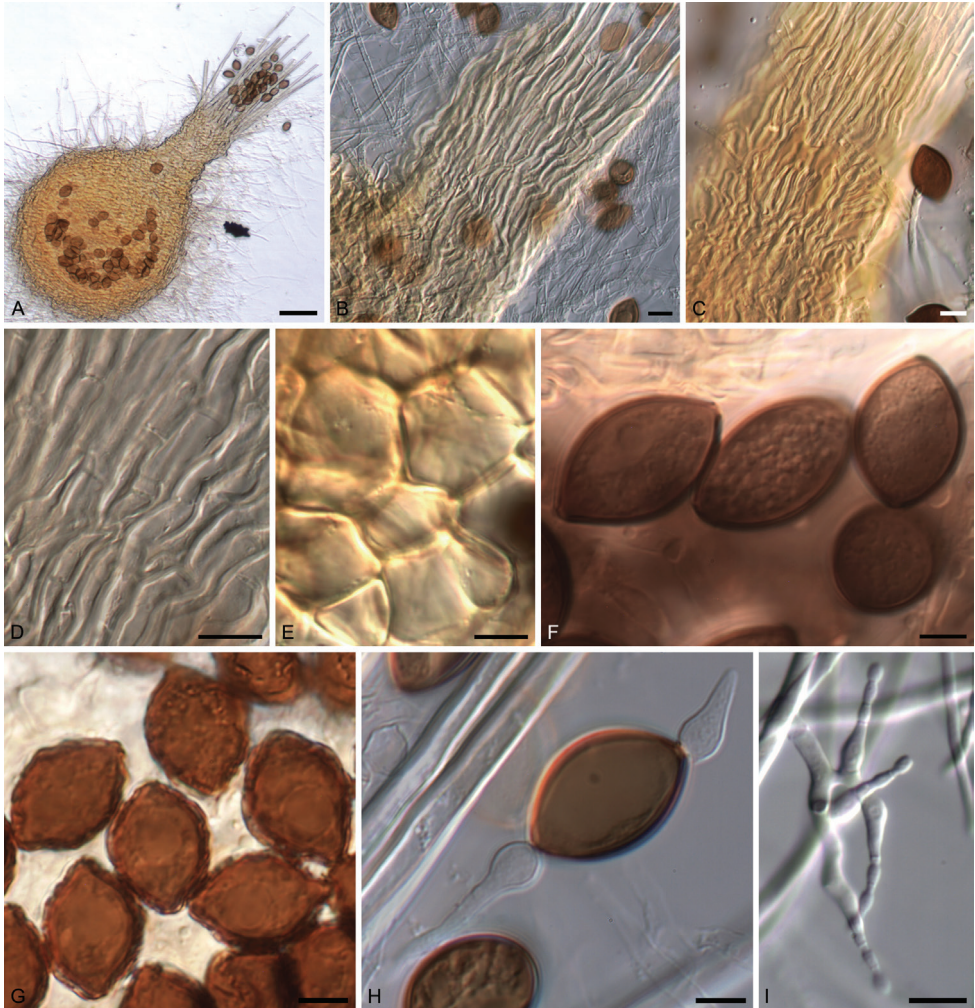
Figure 4. Morphological features of the genus Melanospora . Melanospora dammosa (CBS 113681). A Ascoma B Ascomatal neck D Detail of hyphal neck F Ascospores H Ascospore germinating. Melanospora zamiae (NBRC 7902) C Ascomatal neck E Detail of ascomatal wall. Melanospora verrucispora (NBRC 31375 T ) G Ascospores I Phialidic asexual morph. Scale bars: 50 µm ( A ); 10 µm ( B–E, I ); 5 µm ( F–H ).
