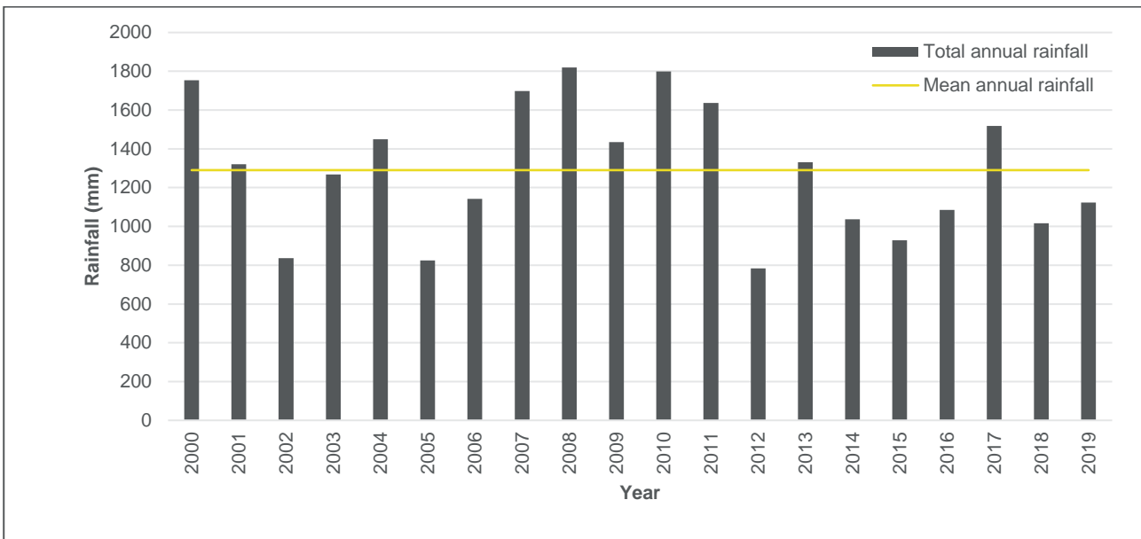
Figure 2-3 Annual Mean Rainfall
