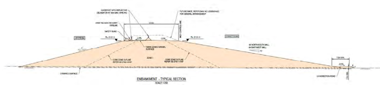
Figure 3 – TSF15 Mine Delivered Embankment - Typical Cross Section
