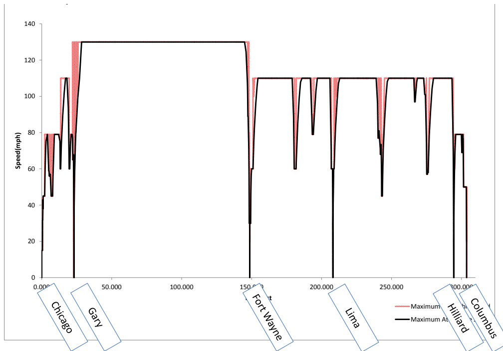
Exhibit 5-3: Chicago to Columbus, Diesel-130, 4-Stop Express in 3:20
