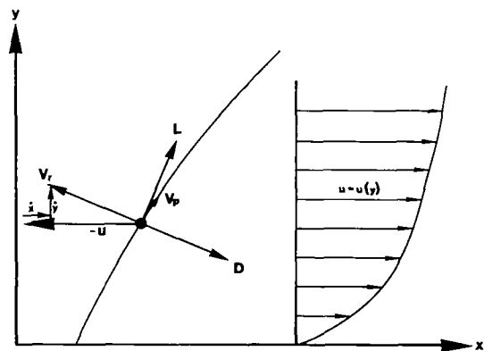
Figure 13. Force diagram for a saltating particle. L denotes lift force; D , drag force; v_p is the instantaneous particle velocity and v_r is the velocity of the particle relative to the wind velocity (modified from White and Schulz, 1977).
