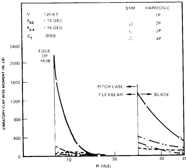
Fig. 34 CFTR - flexbeam harmonic loads
