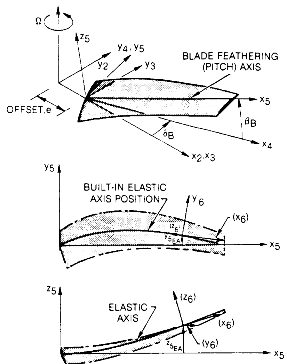
( ) INDICATES PROJECTIONS
