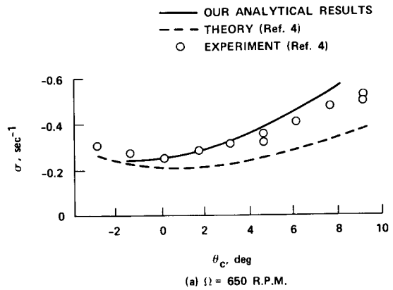
(a) \Omega = 650 R.P.M.
