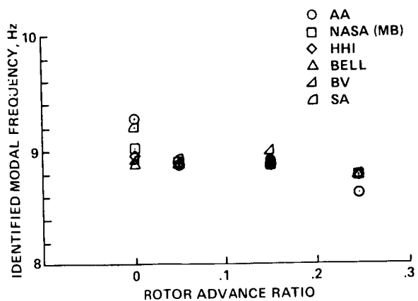
Fig. 12 Identified modal frequency for data set number five; 750 rpm, 222 N lift.
