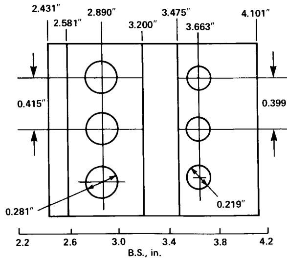
LEAD-LAG FLEXURE
