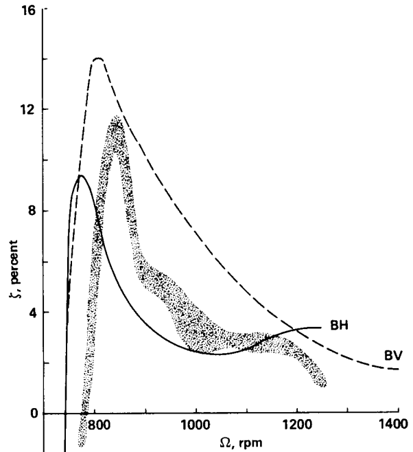
Fig. 7 Composite comparison of theory and experiment for Case 5, regressing lead-lag mode damping as a function of rotor speed for 1 g thrust; \theta_{fh} = 12^\circ , \theta_{bf} = -2.4^\circ , \beta_{pc} = 0^\circ , \beta_d = -2.5^\circ .
