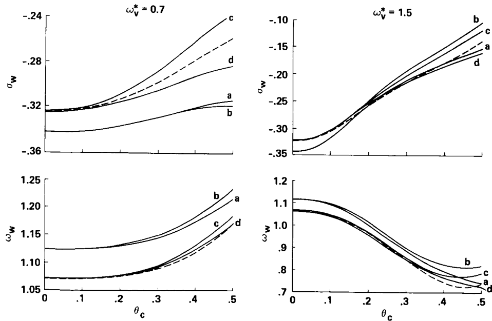
Fig. 8 First flap eigenvalues (real part, \sigma_w , and imaginary part, \omega_w ) versus collective pitch ( \theta_c ) for \omega_w^* = 1.15 , \beta = 0 , \omega_\phi^* = 2.5 , ( N = 5 ).
