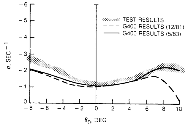
(a) Case 1 - stiff flexure, \beta_B = \Delta\beta = 0 .
