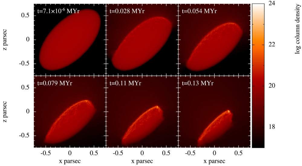
Figure 3. Sequential evolution of the column number density for cloud G1200(5) with the inclination angle \varphi = 45^\circ . Time sequence is left to right, then top to bottom and then left to right.
